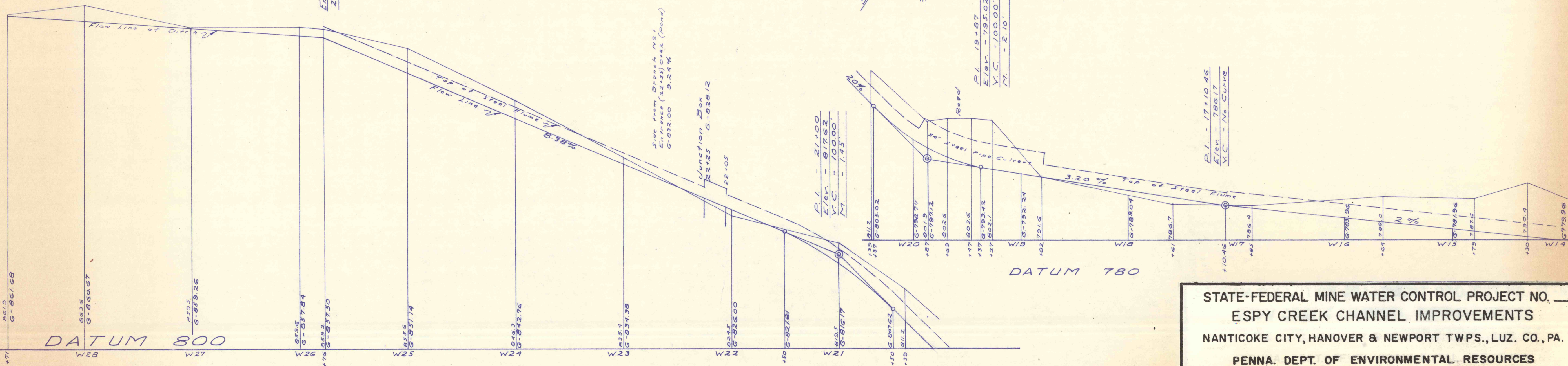
WEST BRANCH - SCALE: HOR. 1"=50' VERT 1"=10'
