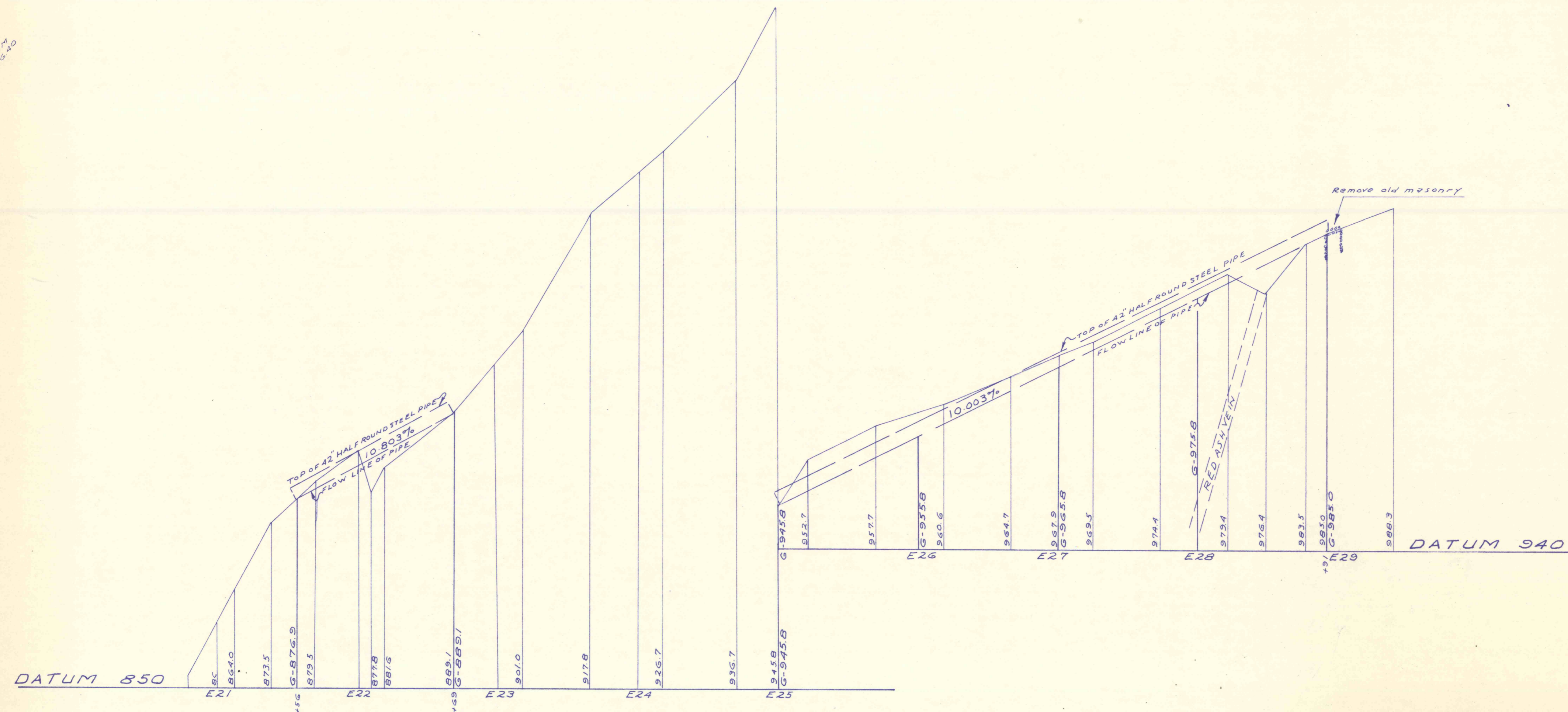
EAST BRANCH PROFILE ALONG \phi OF 42" HALF ROUND STEEL PIPE-LOOKING EAST. SCALE: HOR. 1"=50' VERT. 1"=10'
