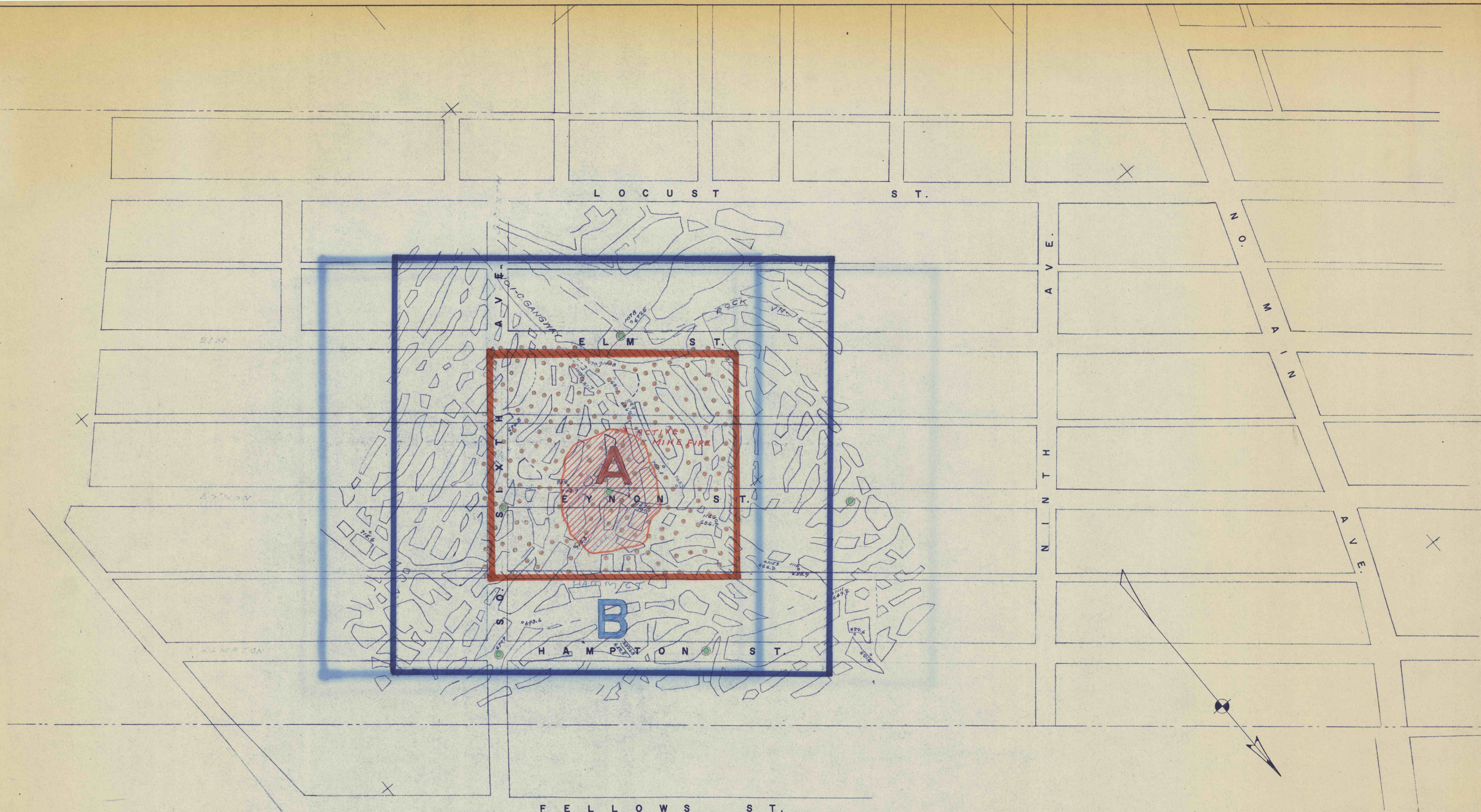
MAP SHOWING DIAMOND VEIN PROPOSED FLUSHING AREAS - TO CONTROL MINE FIRE BELLEVUE SECTION CITY OF SCRANTON, LACKAWANNA CO. PA. PUBLIC HEALTH & SAFETY PROJECT NO. PENNSYLVANIA DEPARTMENT OF MINES & MINERAL IND'S. SCALE - 1" = 100' JULY 1964
