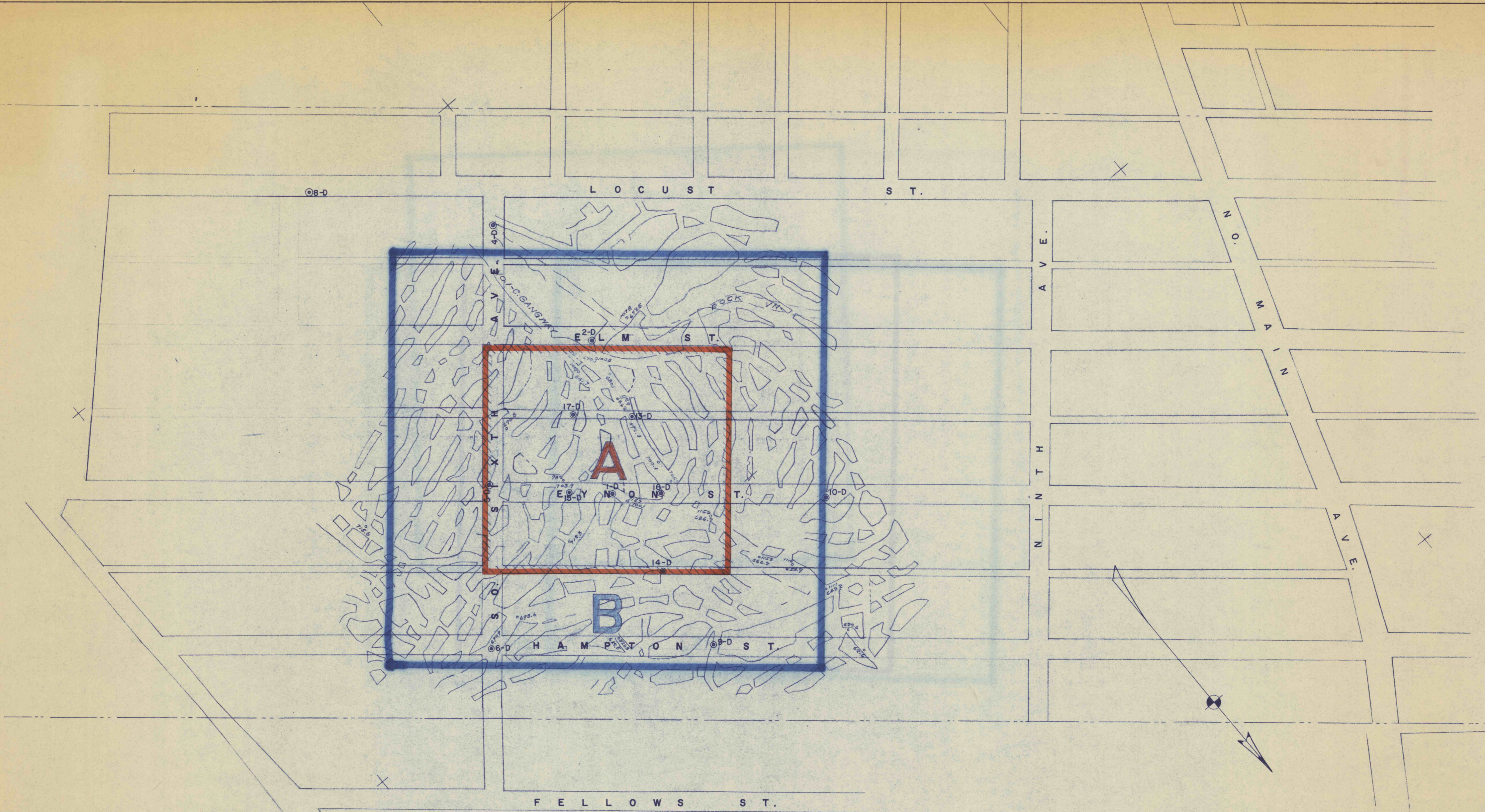
MAP SHOWING DIAMOND VEIN PROPOSED FLUSHING AREAS - TO CONTROL MINE FIRE BELLEVUE SECTION CITY OF SCRANTON, LACKAWANNA CO. PA. PUBLIC HEALTH & SAFETY PROJECT NO. 9 PENNSYLVANIA DEPARTMENT OF MINES & MINERAL IND'S. SCALE - 1" = 100' JULY 1964
