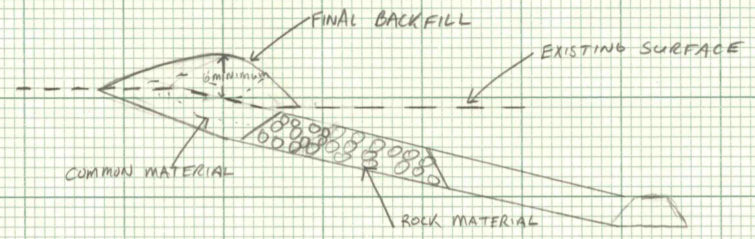
TYPICAL SECTION (FINAL BACKFILL FOR MULEWAY) NOT TO SCALE
