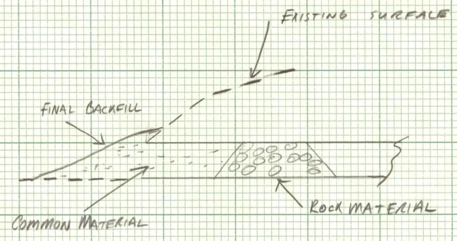
TYPICAL SECTION (FINAL BACKFILL FOR WATER LEVEL TUNNEL) NOT TO SCALE
