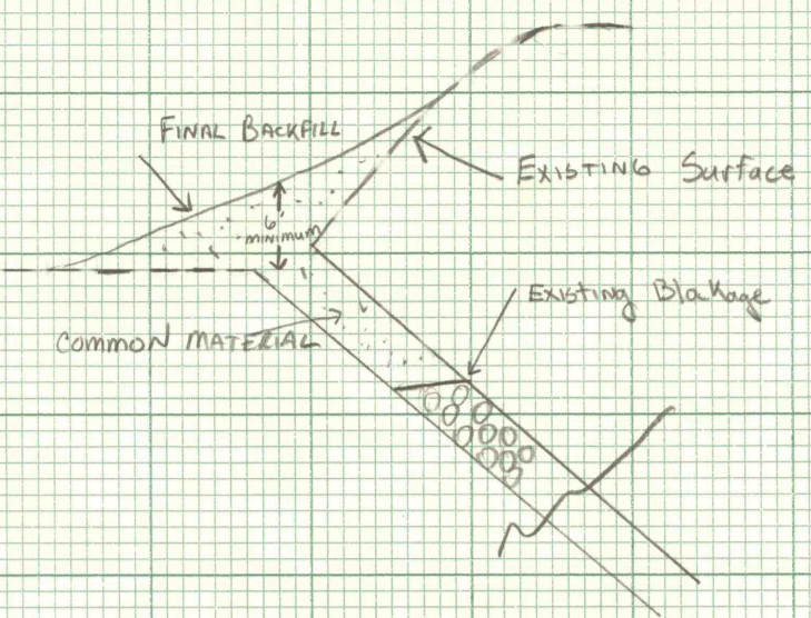
TYPICAL SECTION (Final Backfill for No. 1 Slope, Croppall No. 2, Croppall No. 3 and Airway) NOT TO SCALE
