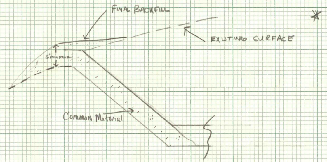
TYPICAL SECTION (FINAL BACKFILL FOR AIRHOLE) NOT TO SCALE
