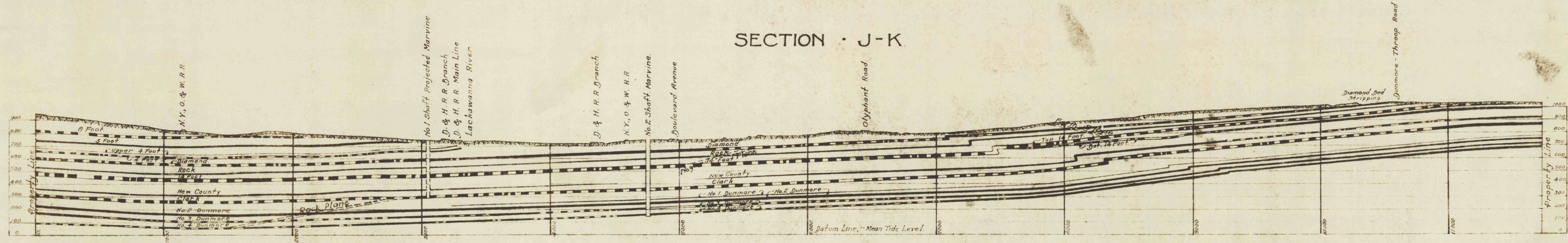
CROSS · SECTIONS THROUGH MARVINE · COLLIERY Scale 1" = 400'
