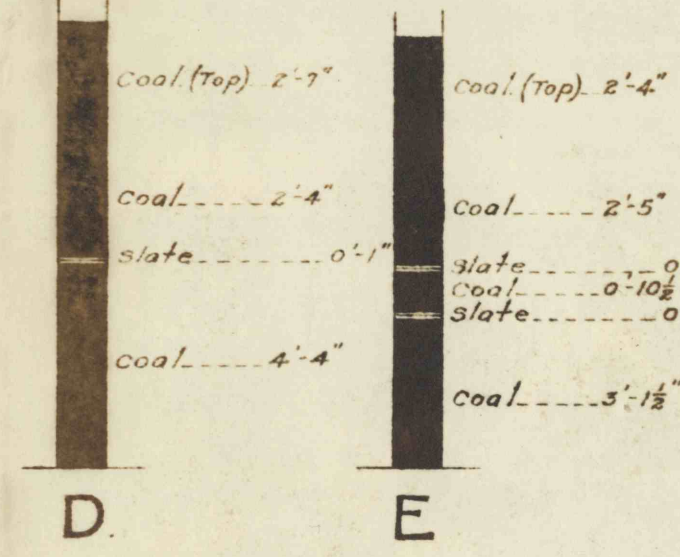
BED SECTIONS
