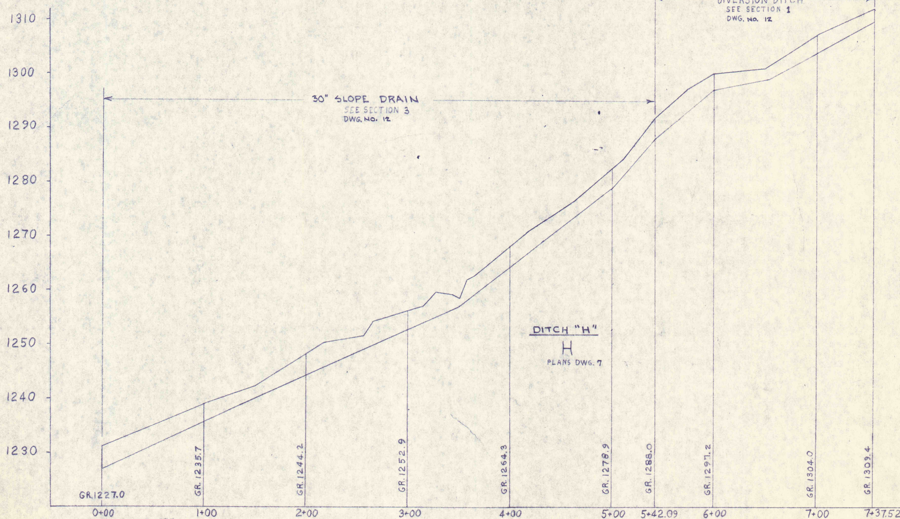
PROFILES OF DITCHES G & H SCALE = HORIZONTAL - 1" = 50' VERTICAL - 1" = 10'
