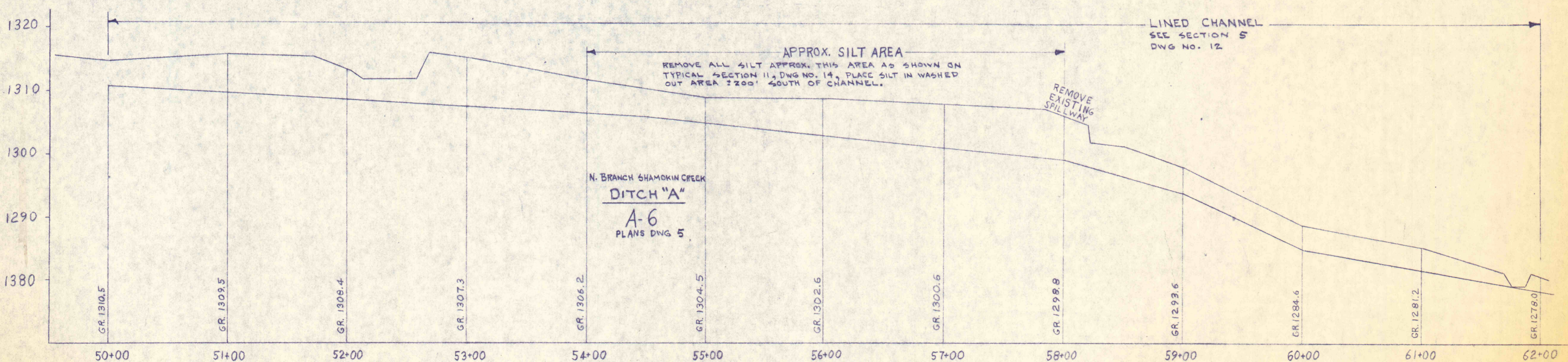
PROFILES OF DITCH A SCALE = HORIZONTAL - 1" = 50' VERTICAL - 1" = 10'
