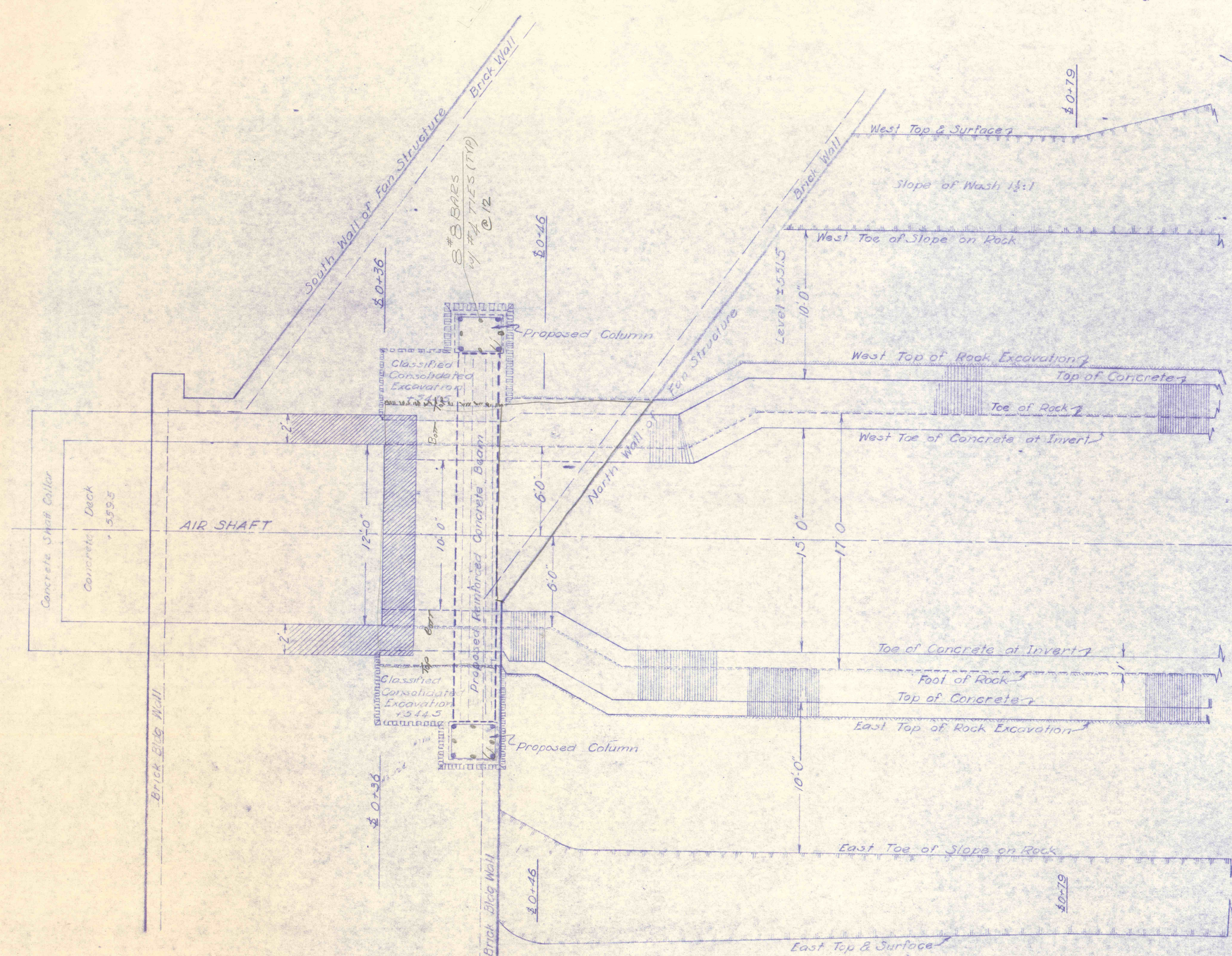
PLAN Vicinity of Shaft
