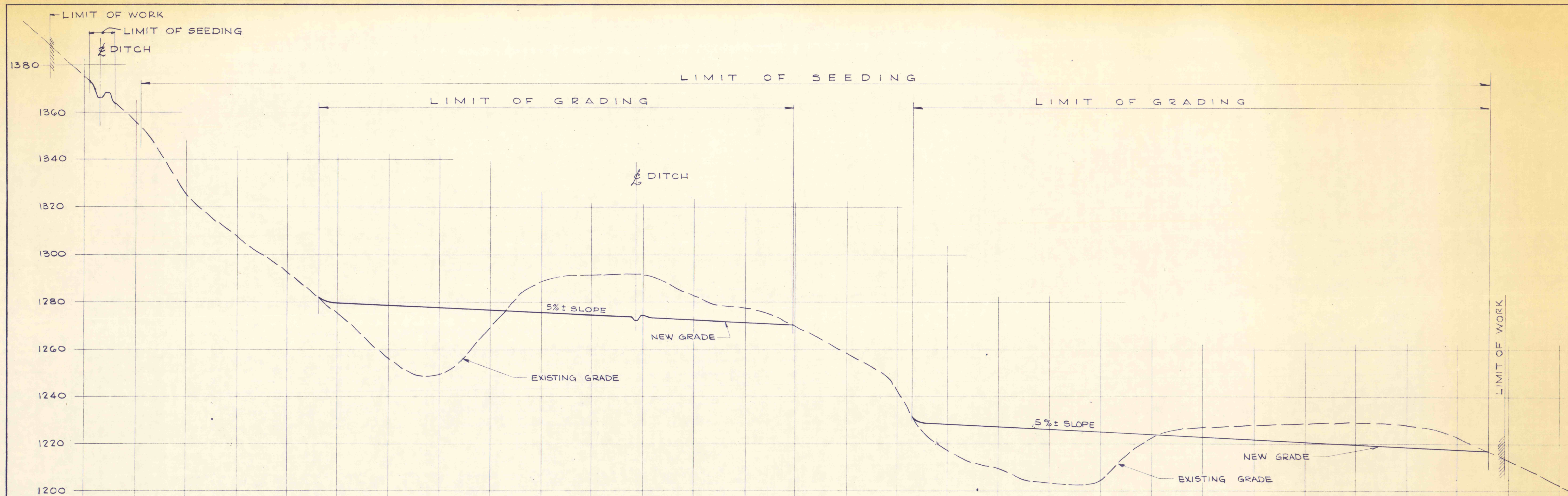
CROSS-SECTION NO. 3 SCALE: 1" = 20' (HORIZ. & VERT.) FOR LOCATION SEE DRAWING NO. 2
