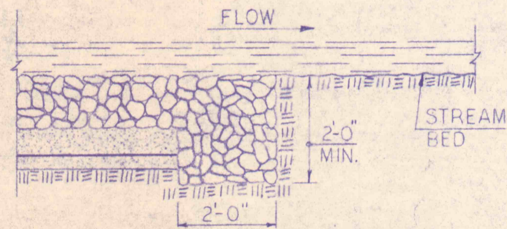
RIP RAP CUTOFF DETAIL STA. 24+64.13
