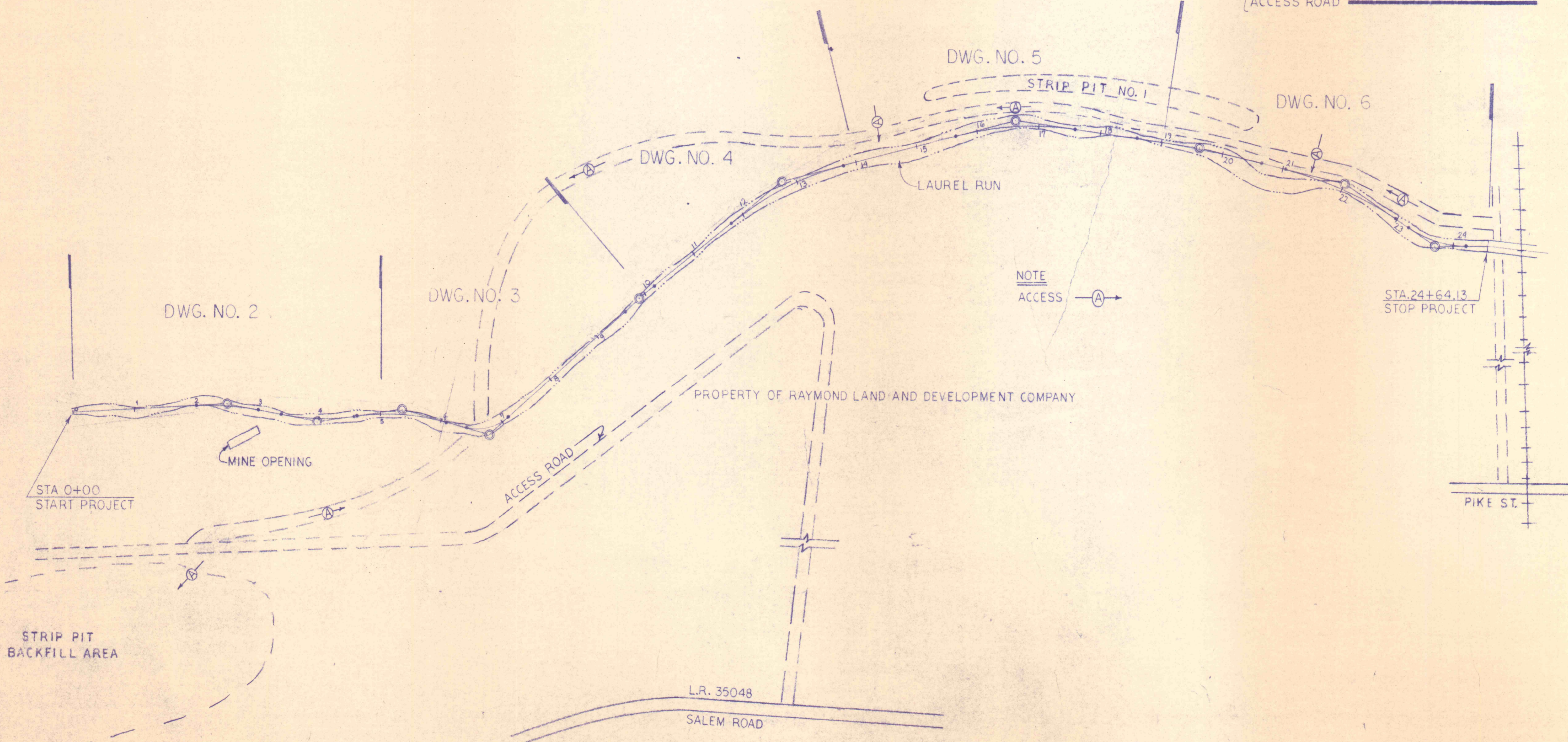
GENERAL PLAN OF CHANNEL RESTORATION SCALE: 1"=100'
