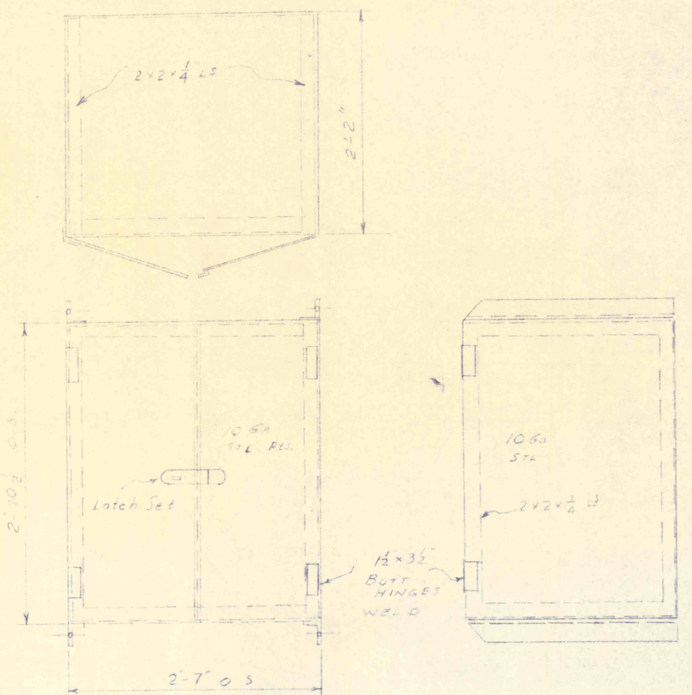
5-DAY OILER CABINET ALL WELDED CONSTRUCTION ONE REQD - R-180418 SCALE 1"=10"
