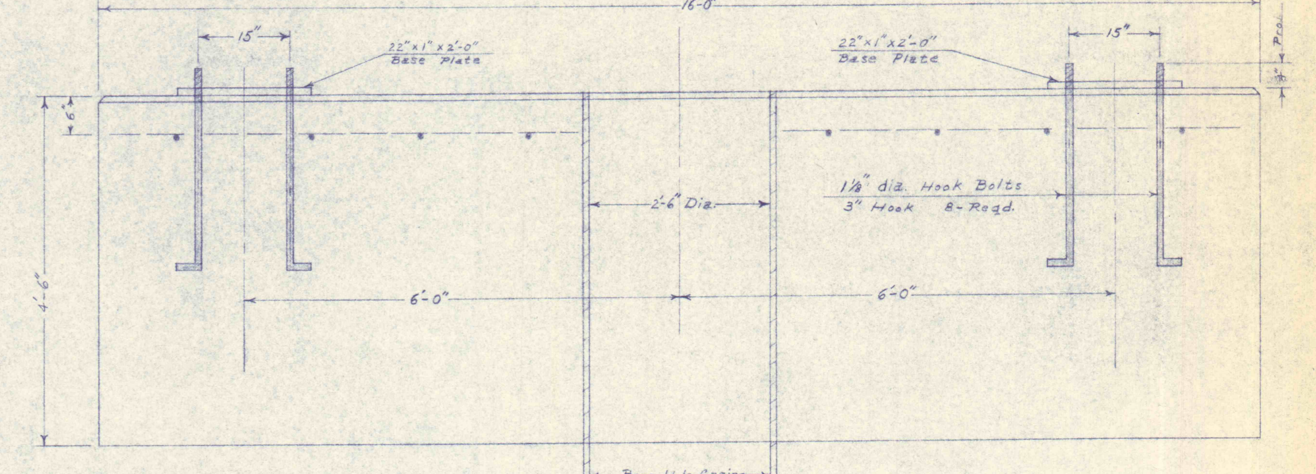
Longitudinal Sect. A-A Tower Pier-X HEADFRAME & PUMP FOUNDATION scale 3/4"=1'
