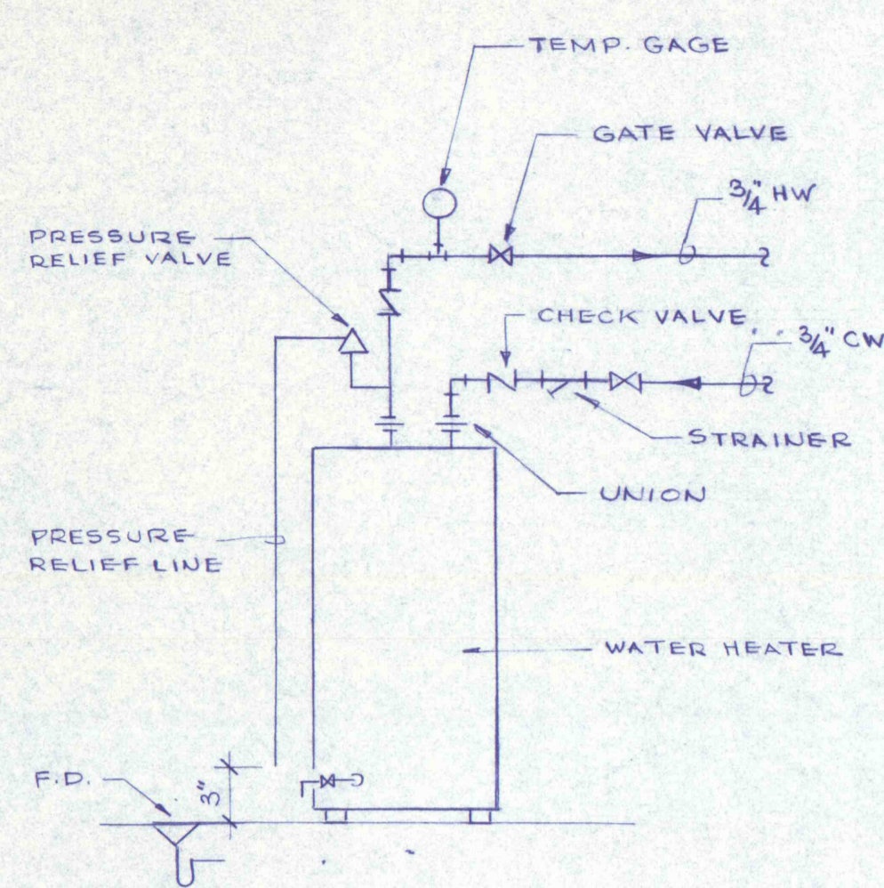
ELECTRIC WATER HEATER PIPING ARRGT. NTS
