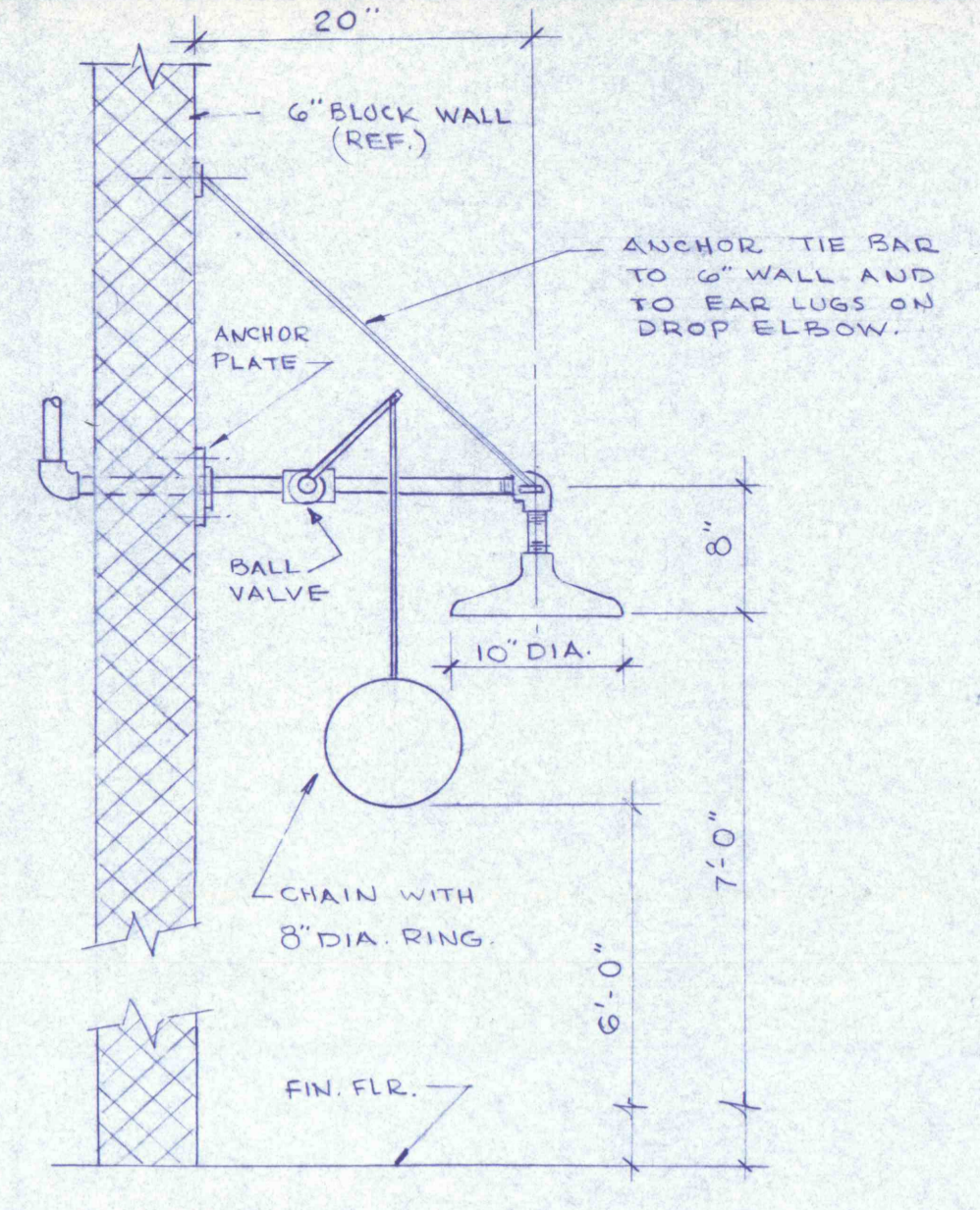
EMERGENCY SHOWER (F7) DETAIL SCALE: 1/2" = 1'-0"
