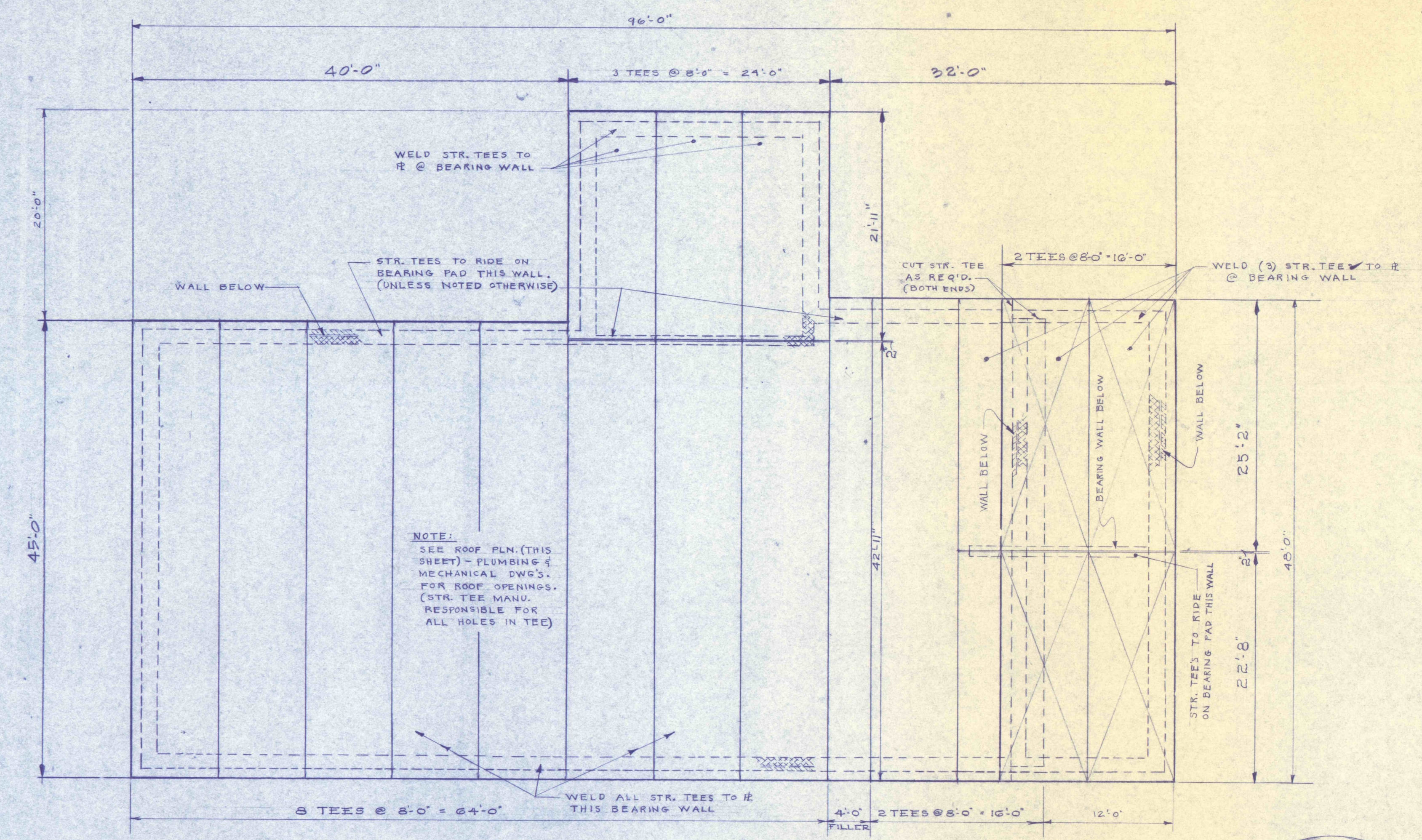
ROOF FRAMING PLAN SCALE: 1/8" = 1'-0"
