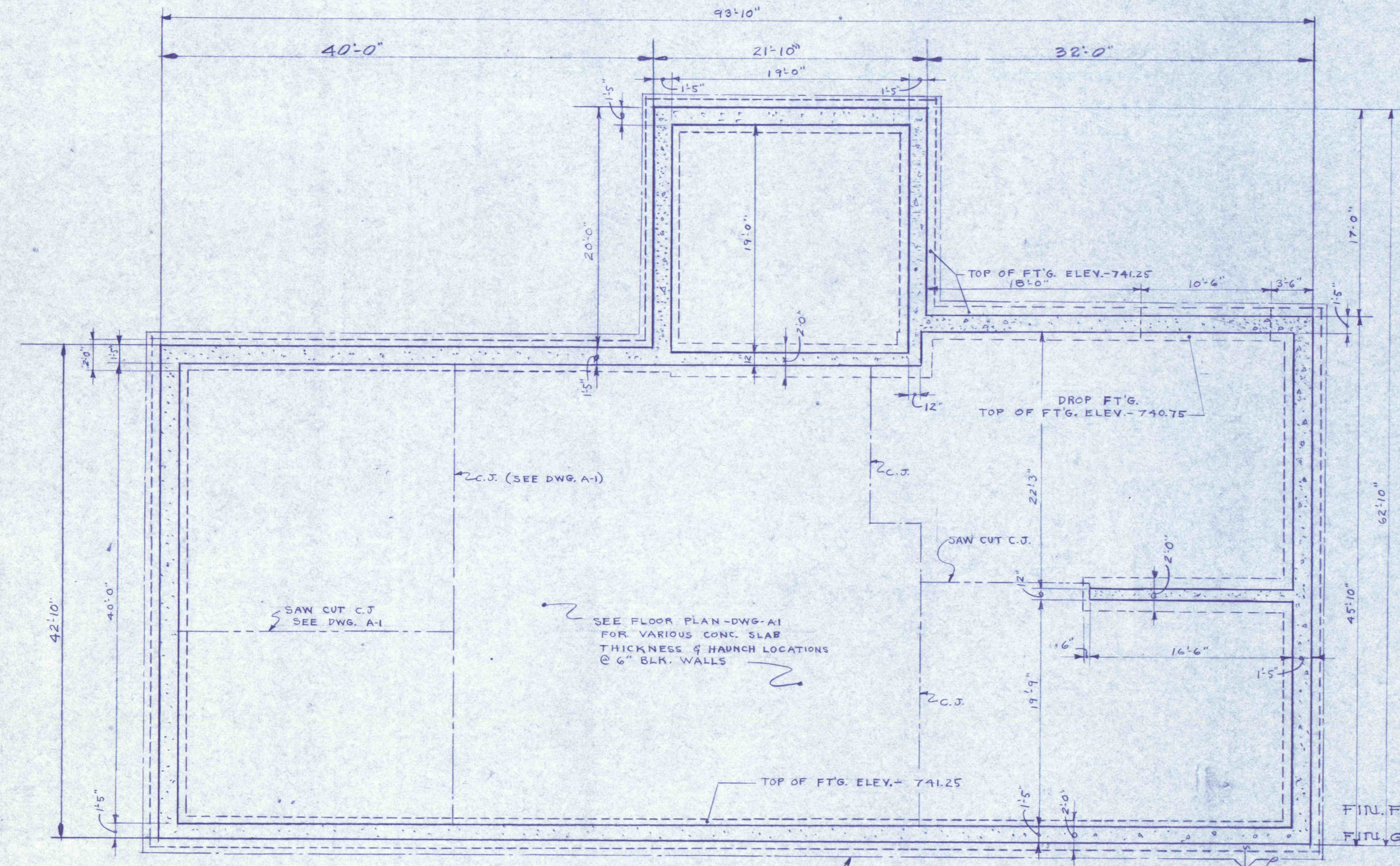
FOUNDATION PLAN SCALE: 1/8" = 1'-0"
