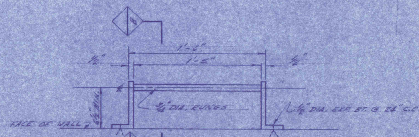
SHIP'S LADDER PLAN SCALE: 1/2" = 1'-0"
