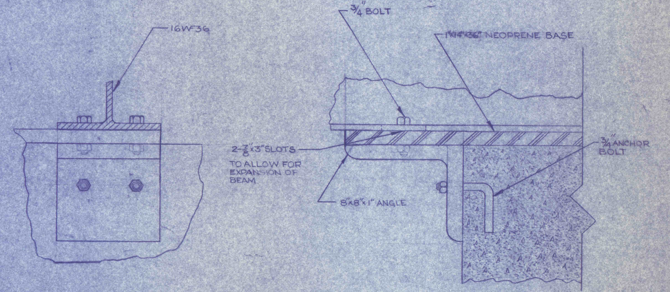
DETAIL C SCALE 1/4" = 1'
