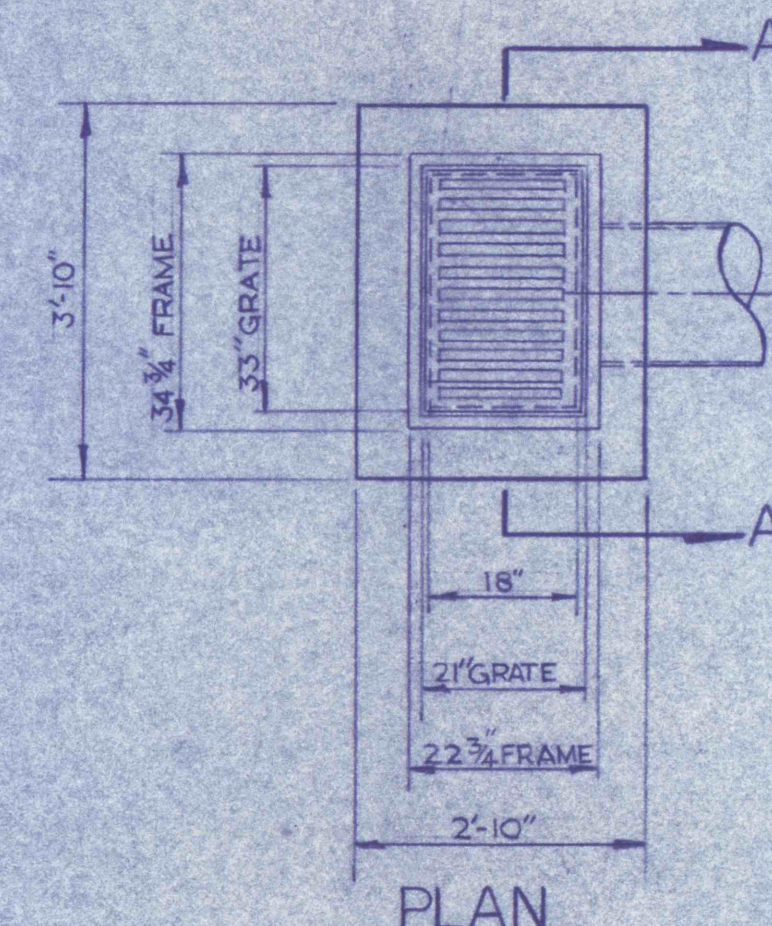
CATCH BASIN DETAIL
