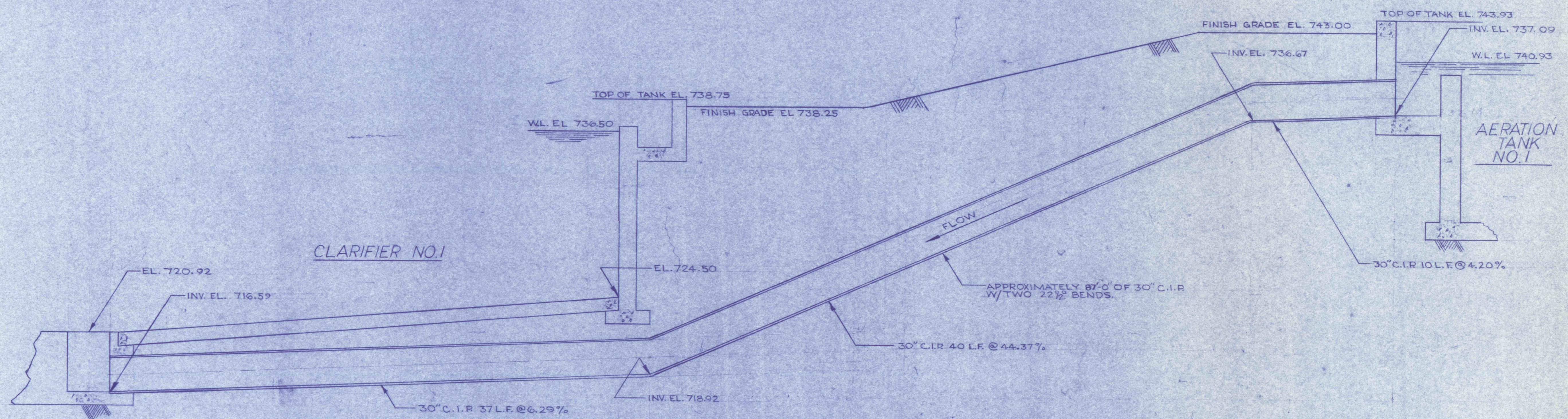
SECTION A-A SCALE 1/4"=1'-0" SEE PIPING LAYOUT PLAN C-4/C-5
