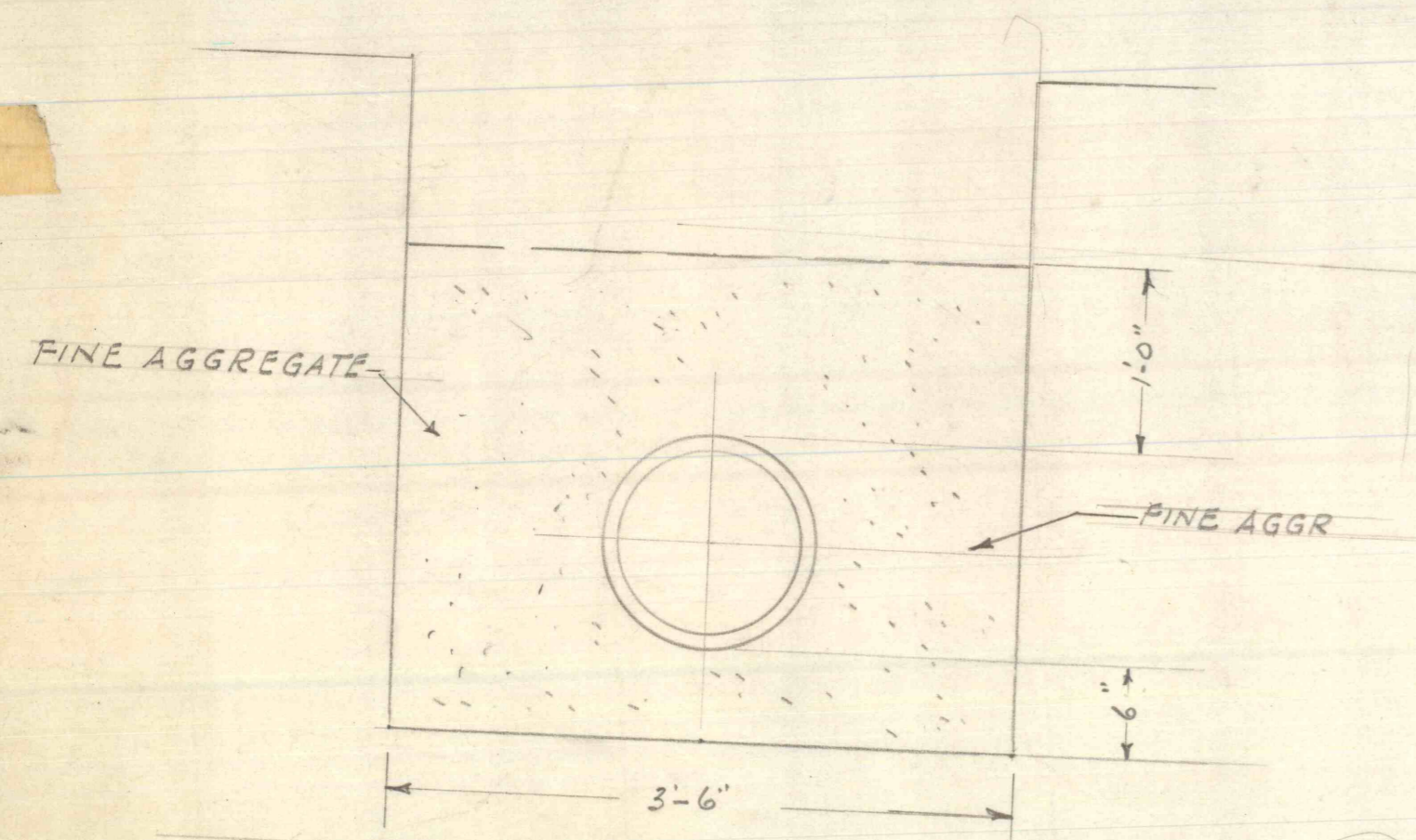
TYPICAL PIPE TRENCH
