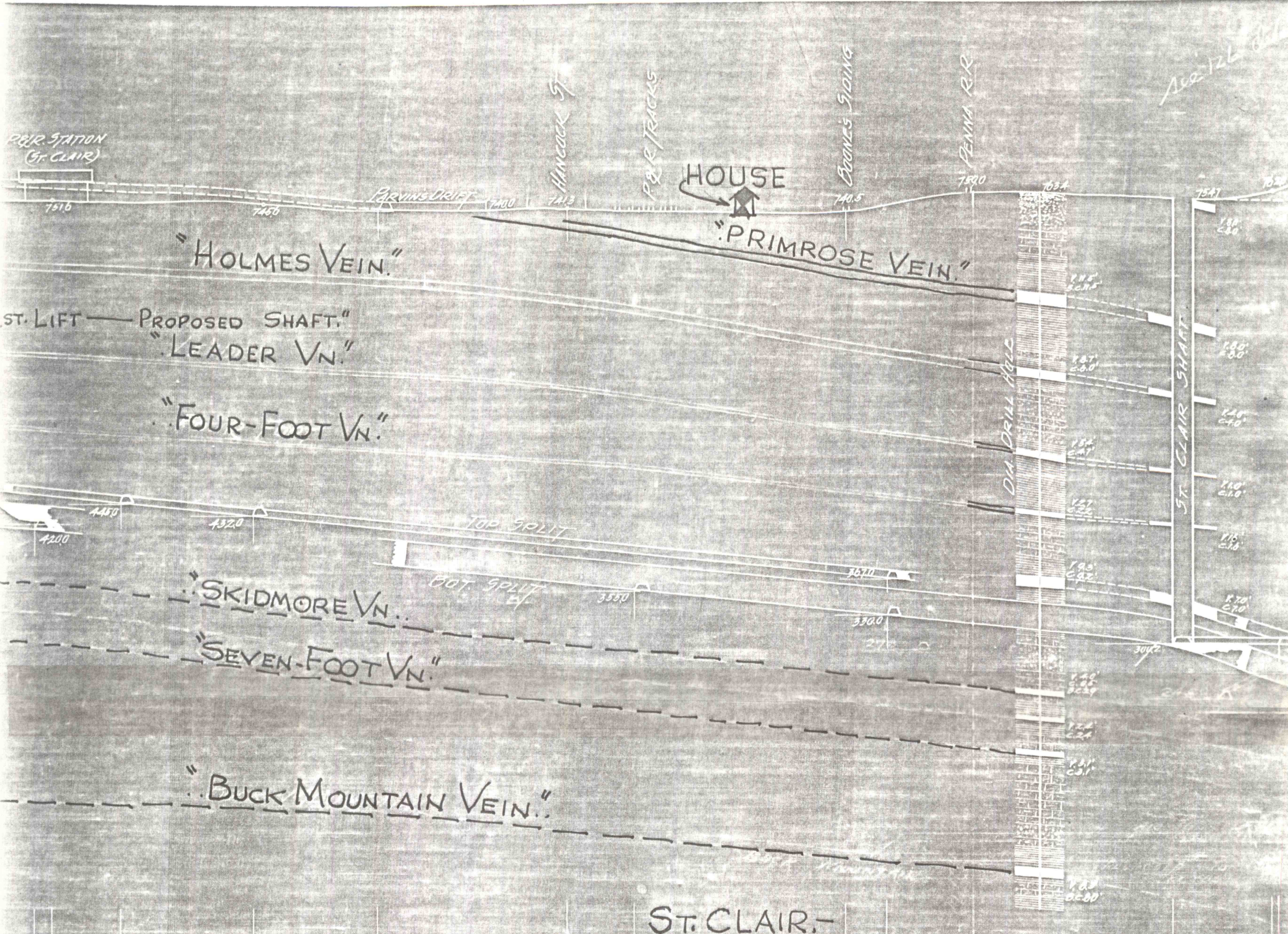
SOUTHERN COAL FIELD. WADESVILLE COLLIERY "X" SECTION No. 5. No. 5 EAST NORWEGIAN TWP, SCHUYLKILL COUNTY, PA, READING ANTHRACITE COLLIERIES.
