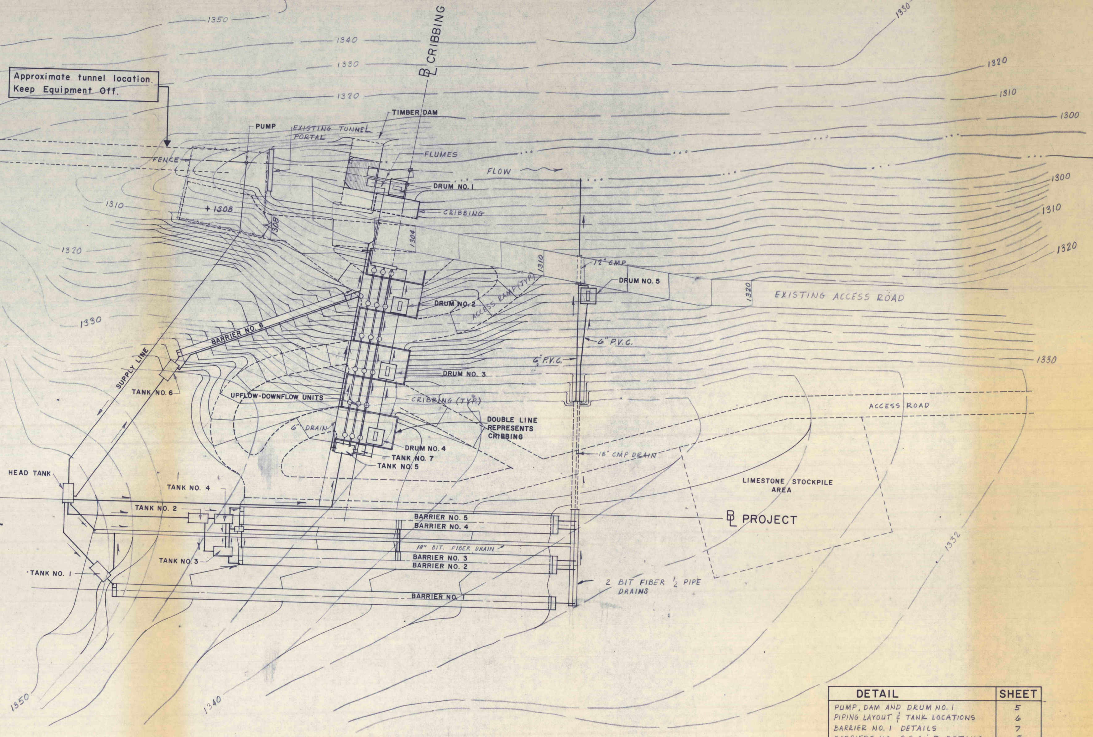
GENERAL PLAN SCALE: 1" = 20'
