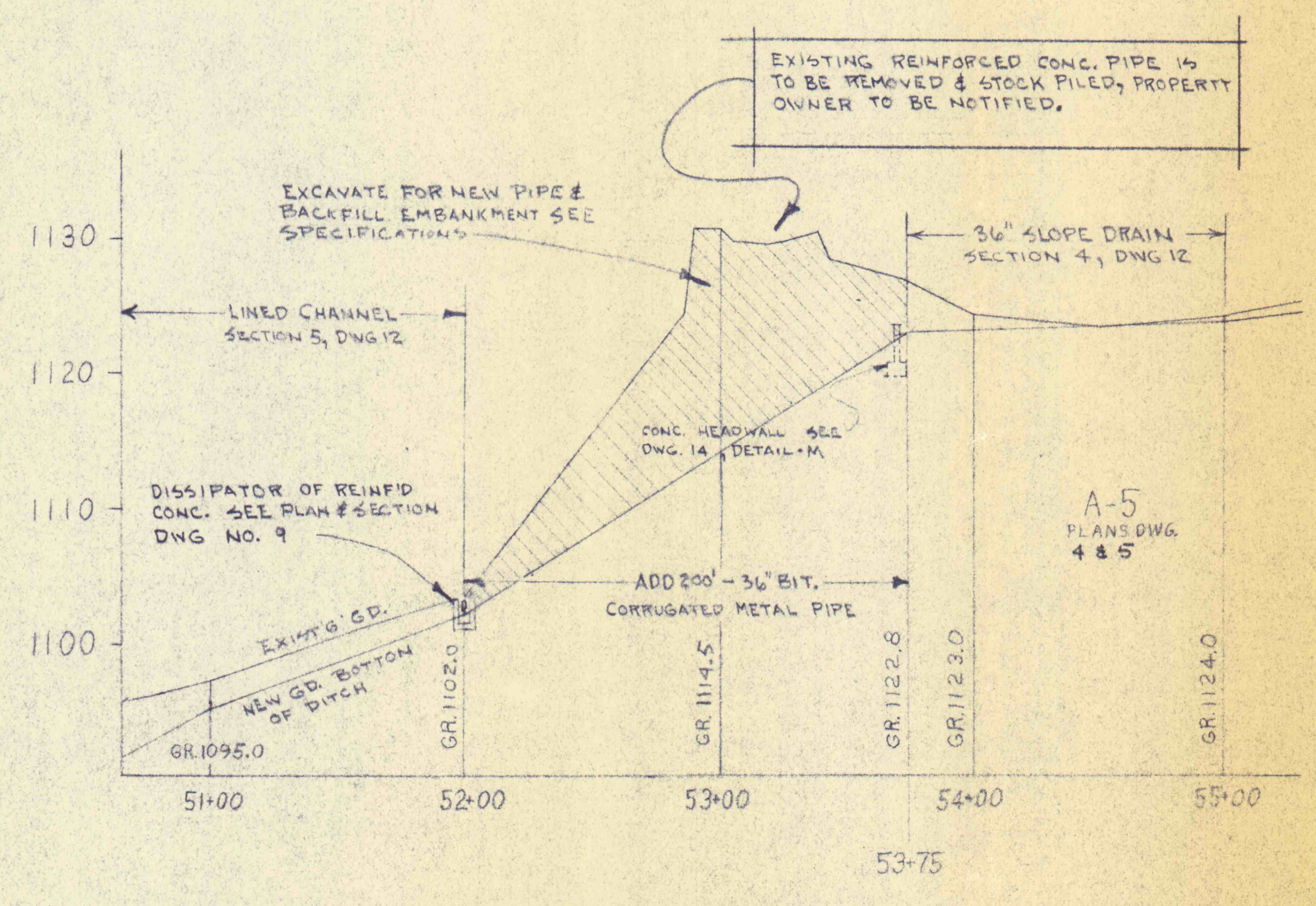
PROFILES OF DITCH "A" SCALE - HORIZONTAL - 1" = 50' VERTICAL - 1" = 10'
