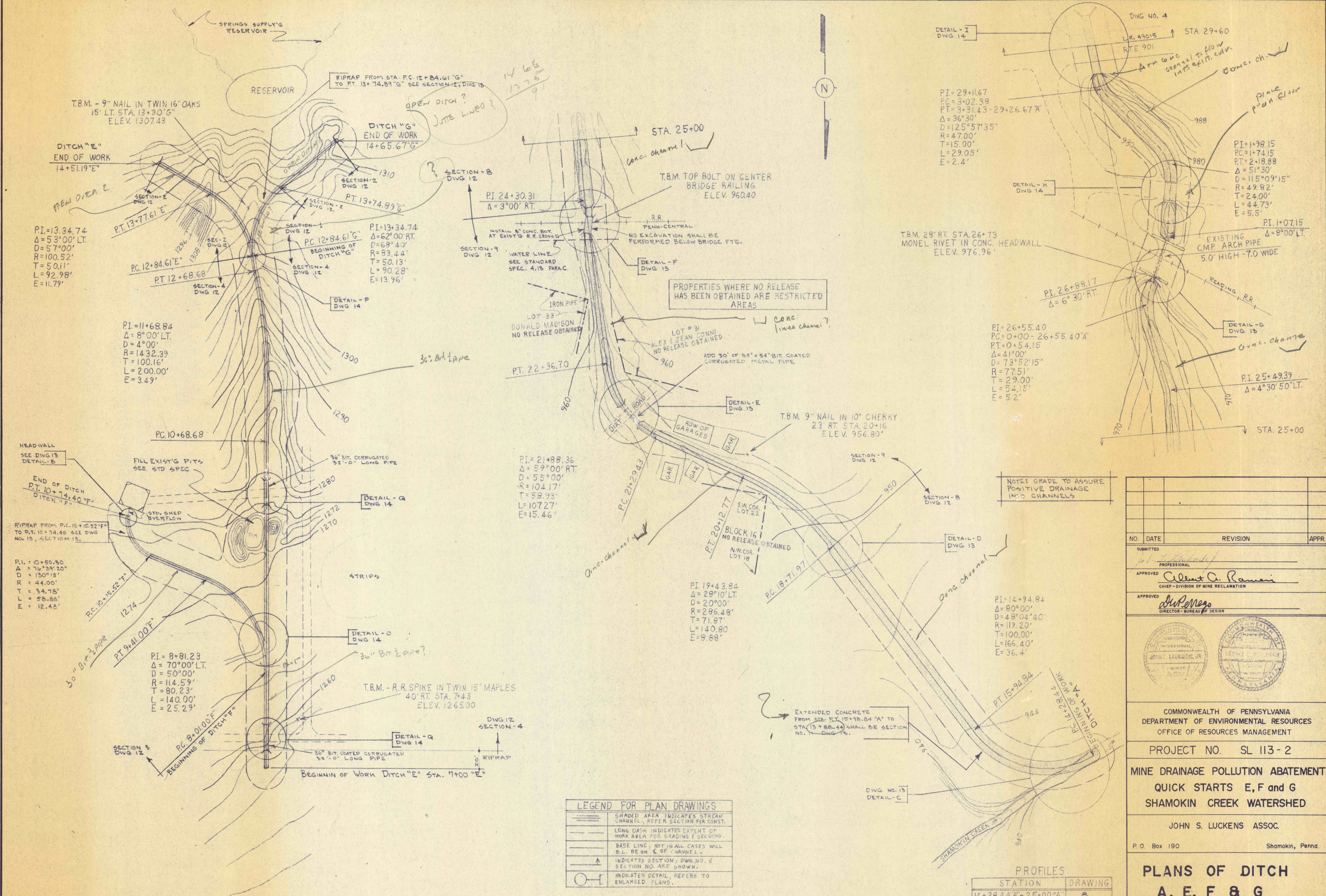
PLANS OF DITCH "A", "E", "F" & "G" SCALE = 1" = 50' - 0"
