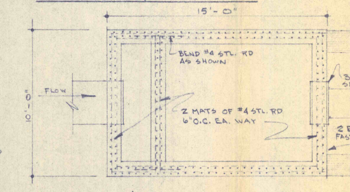
PLAN OF DISSIPATOR DITCH "A" (STA 52+00) SCALE = 1/4" = 1' - 0"
