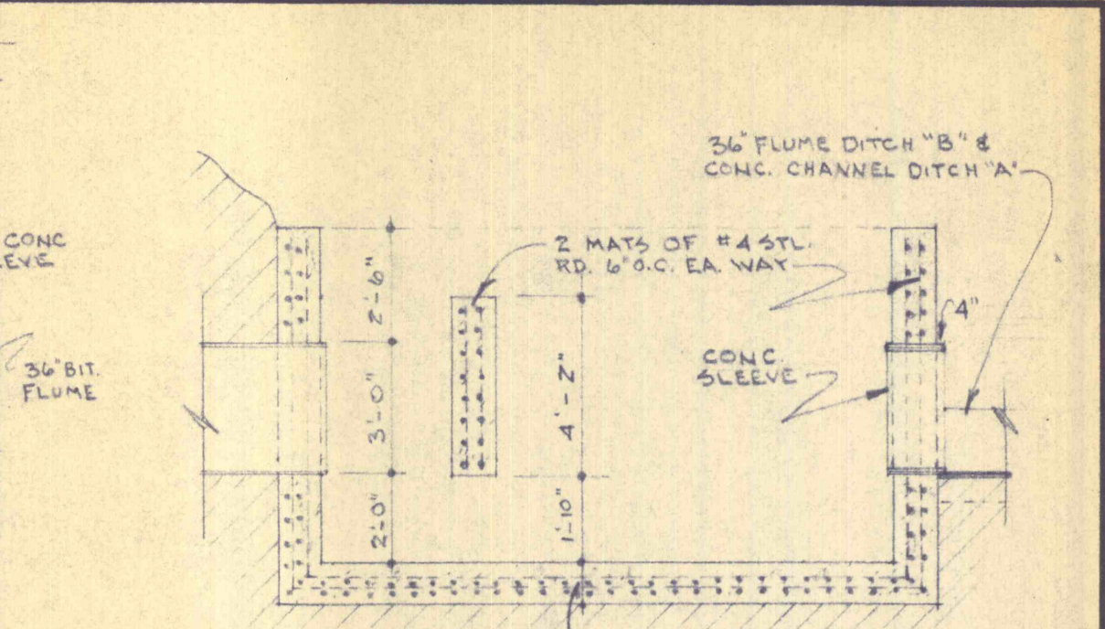
TYP. SECTION OF DISSIPATOR FOR DITCH "A" & "B" SCALE = 1/4" = 1' - 0"
