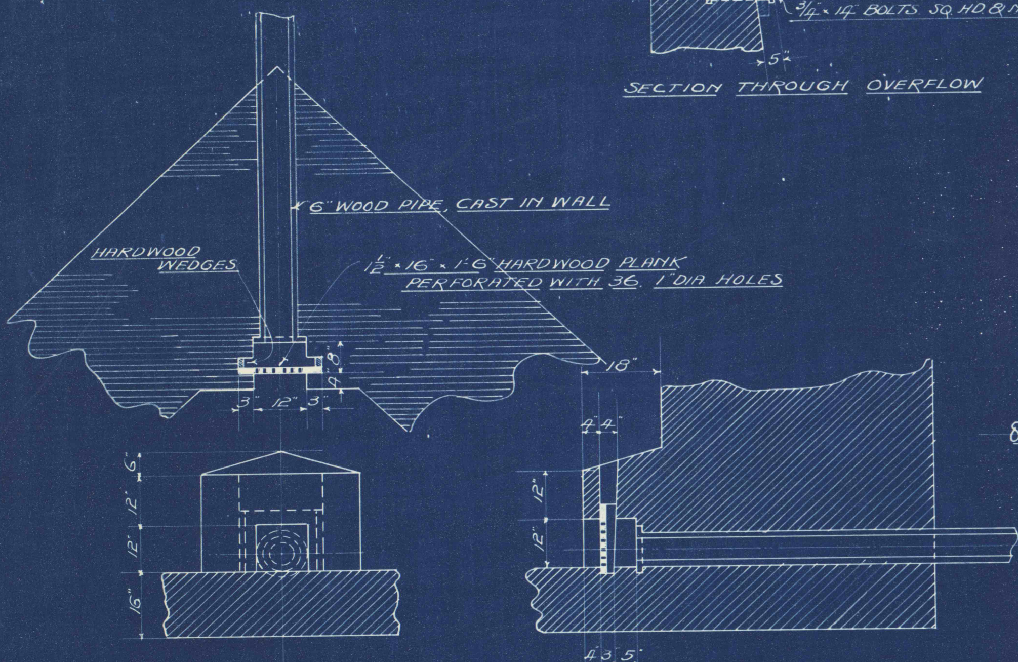
DETAIL OF OUTLET
