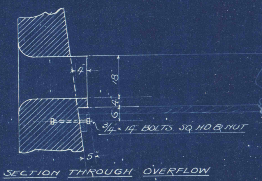
SECTION THROUGH OVERFLOW
