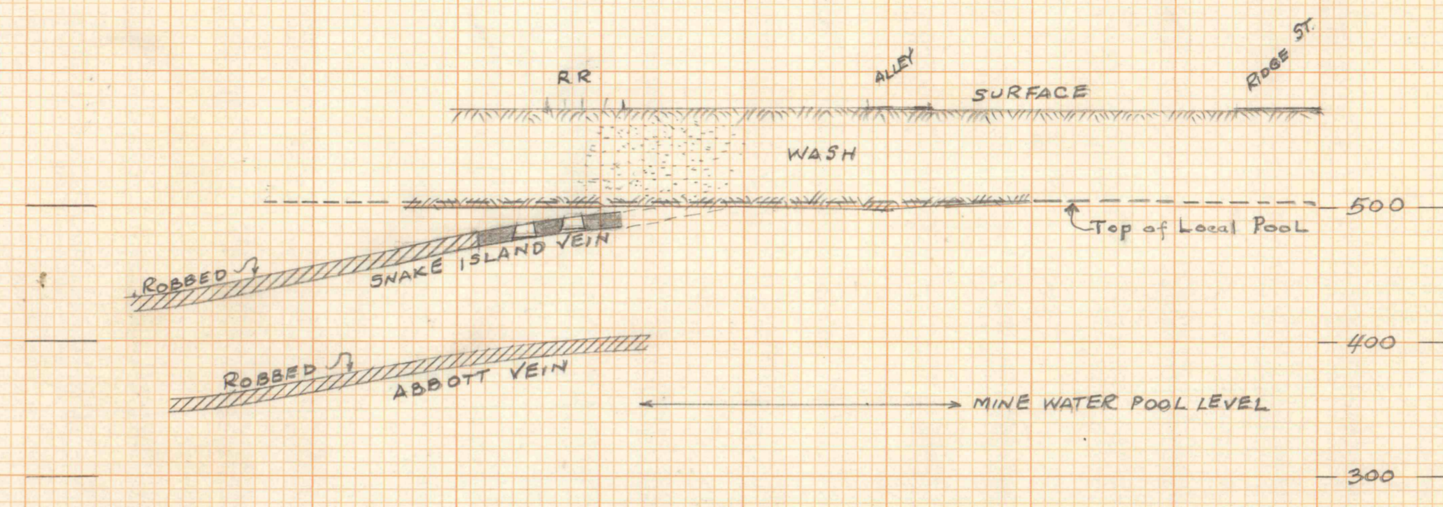
SECTION "A"
