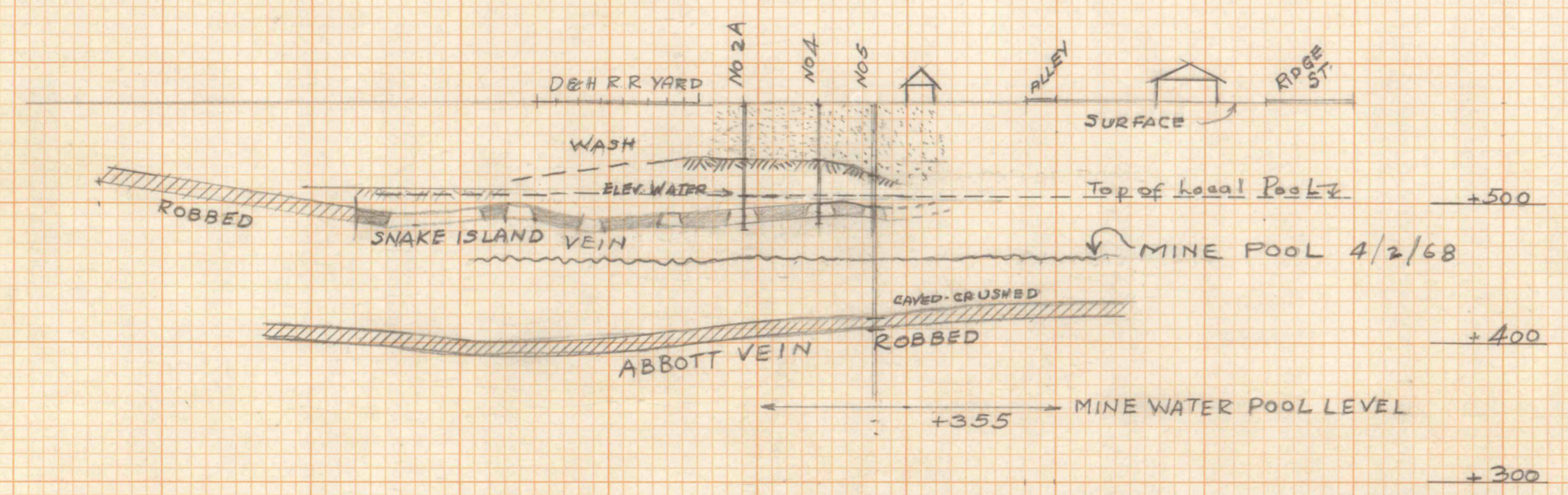
SECTION "C"
