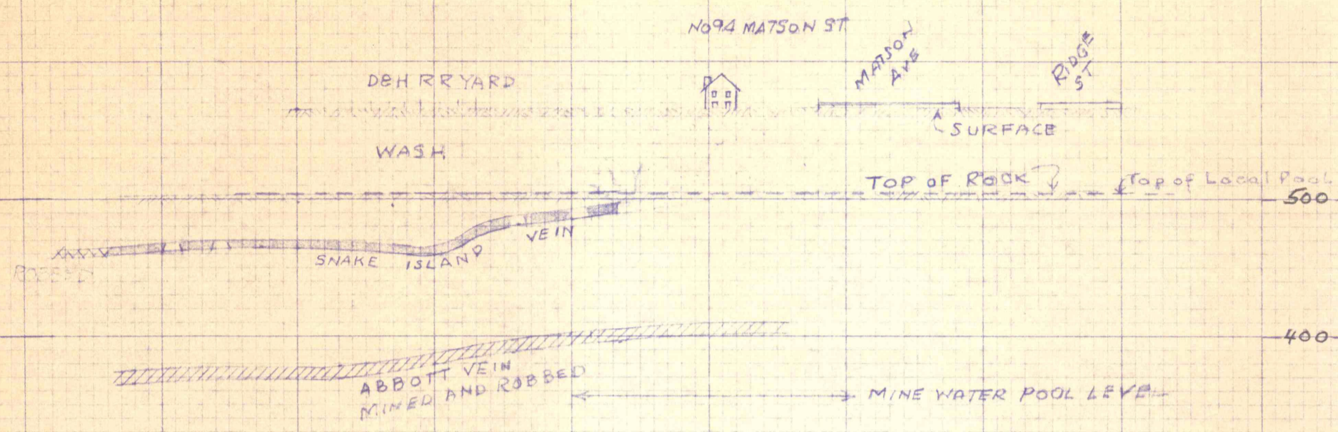
"X" SECTION NW-SE THROUGH #94 MATSON ST PARSONS SECTION OF WILKES-BARRE, PA LOOKING N.E. SECTION "B"
