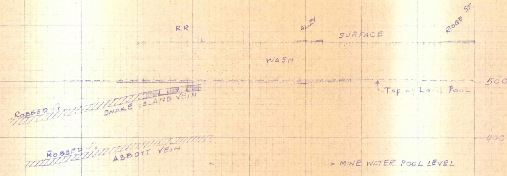
SECTION "A"
