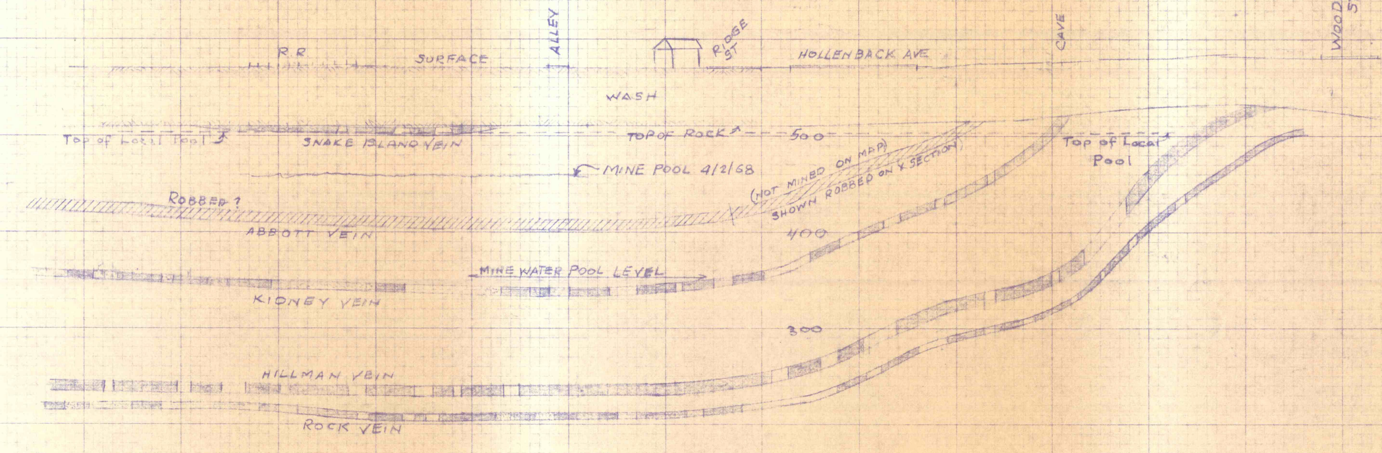
SECTION "D"
