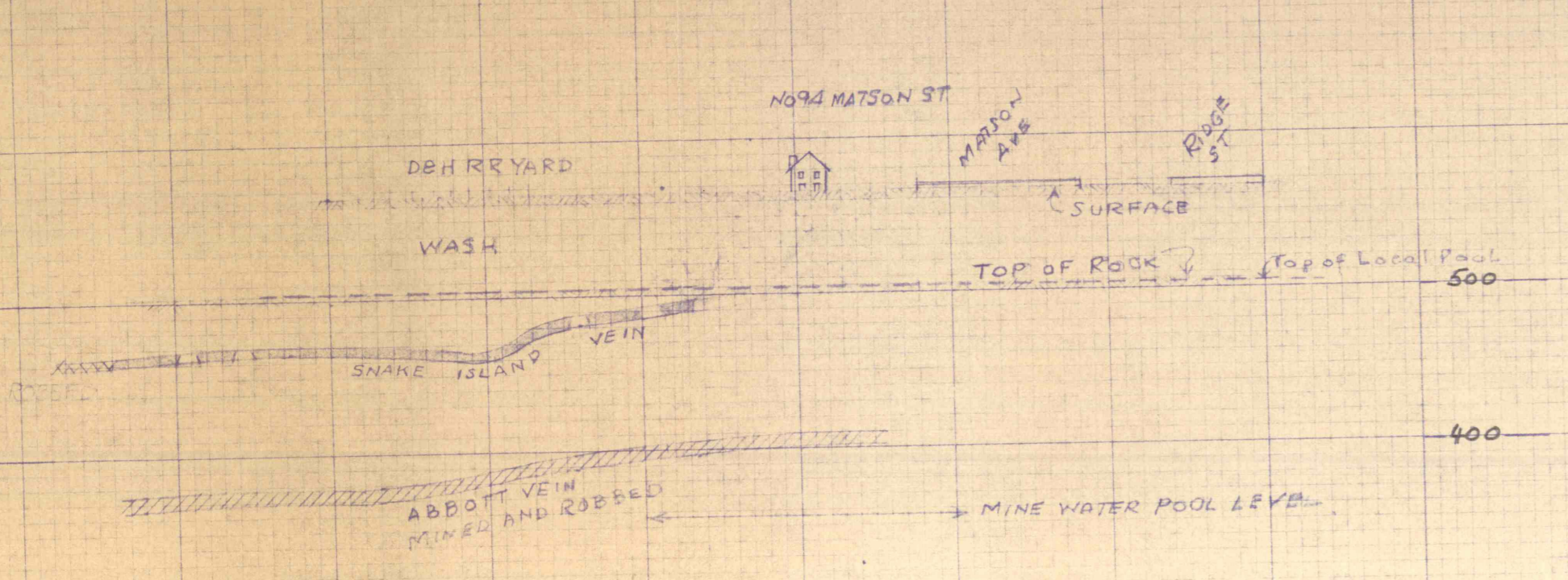
"X" SECTION NW-S.E THROUGH #94 MATSON ST PARSONS SECTION OF WILKES-BARRE, PA LOOKING N.E SECTION "B"
