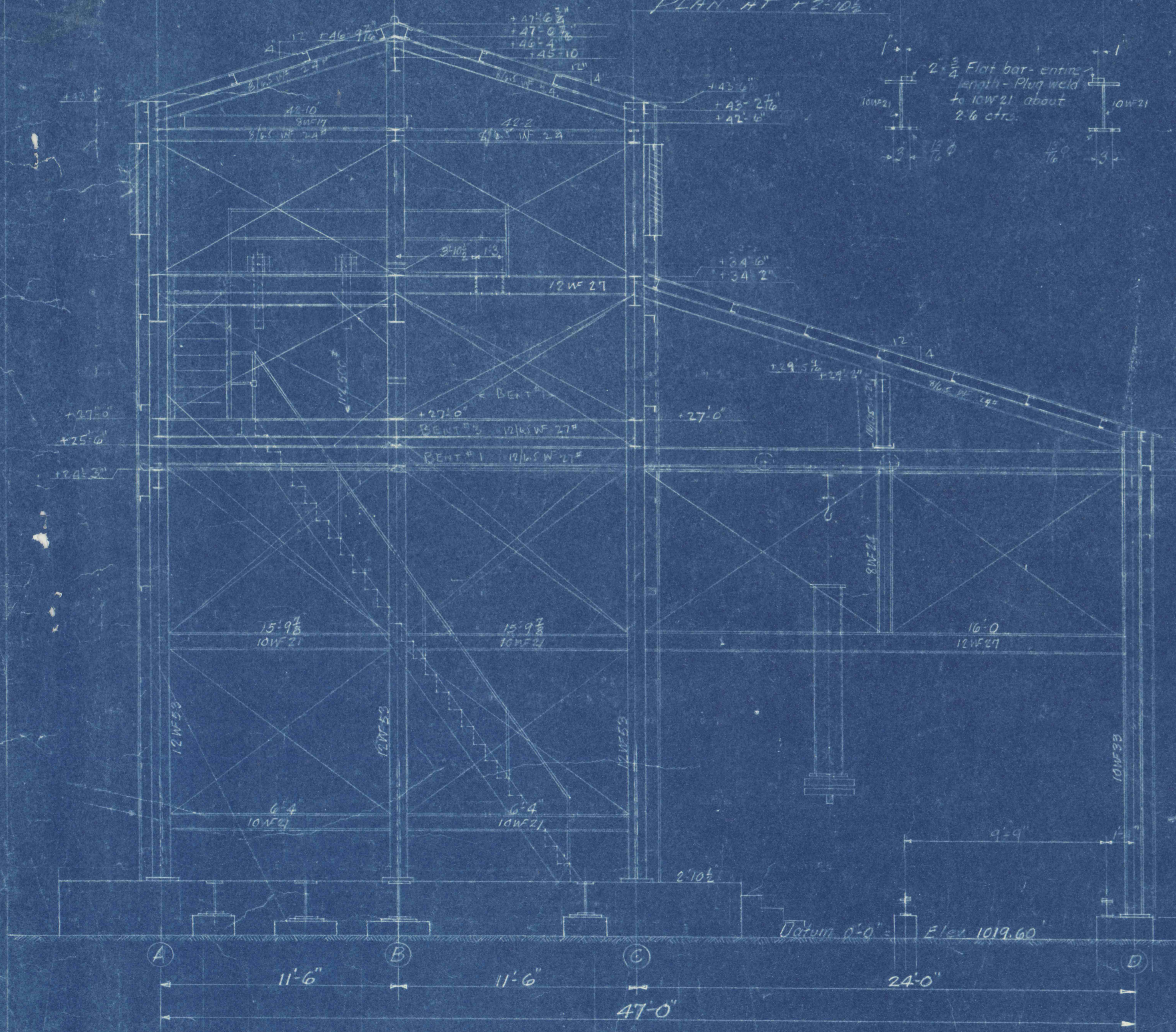
SIDE ELEVATION Scale 1/4"=1'-0"
