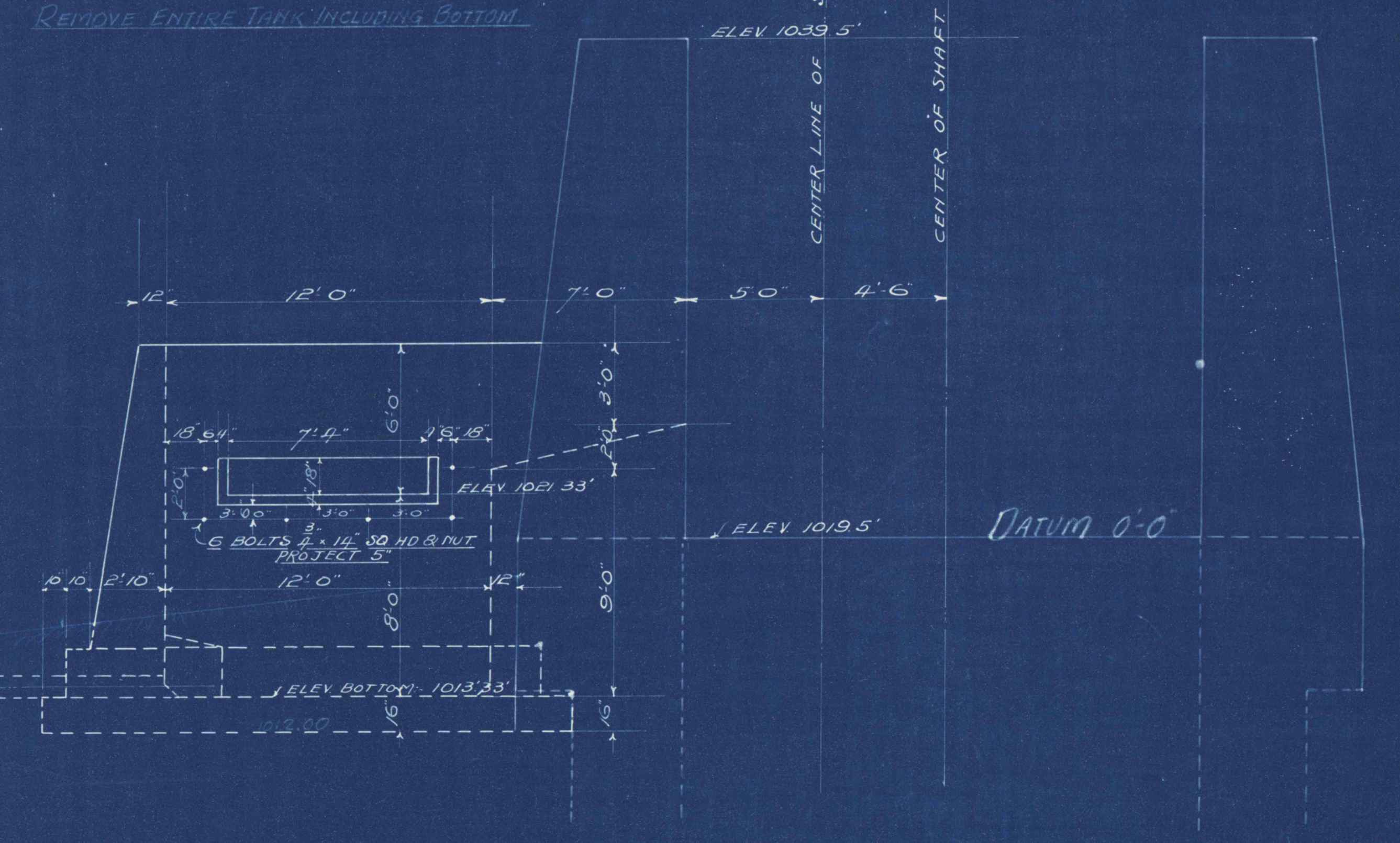
SECTION THROUGH OVERFLOW
