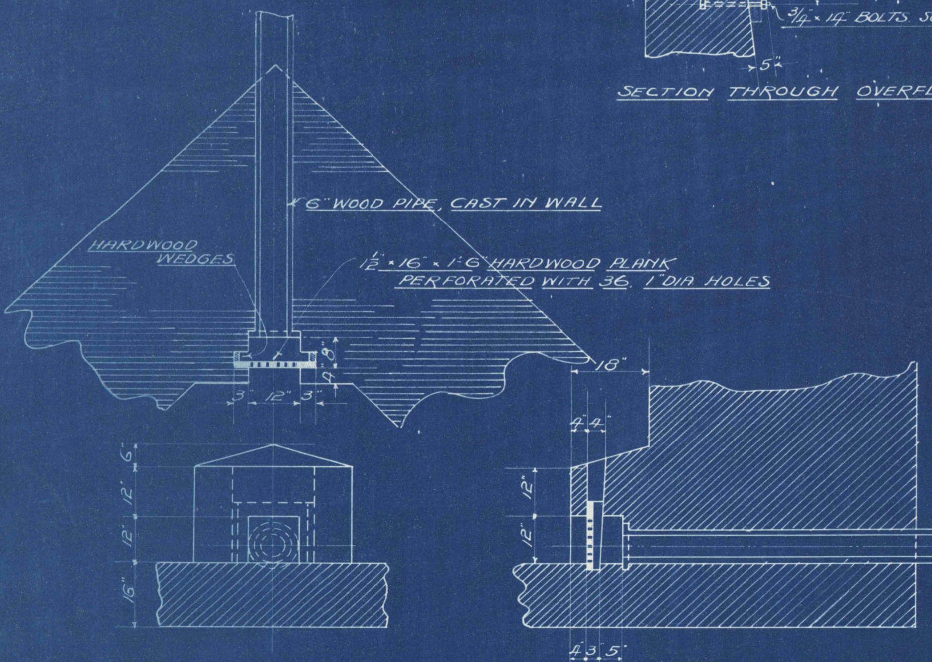
DETAIL OF OUTLET
