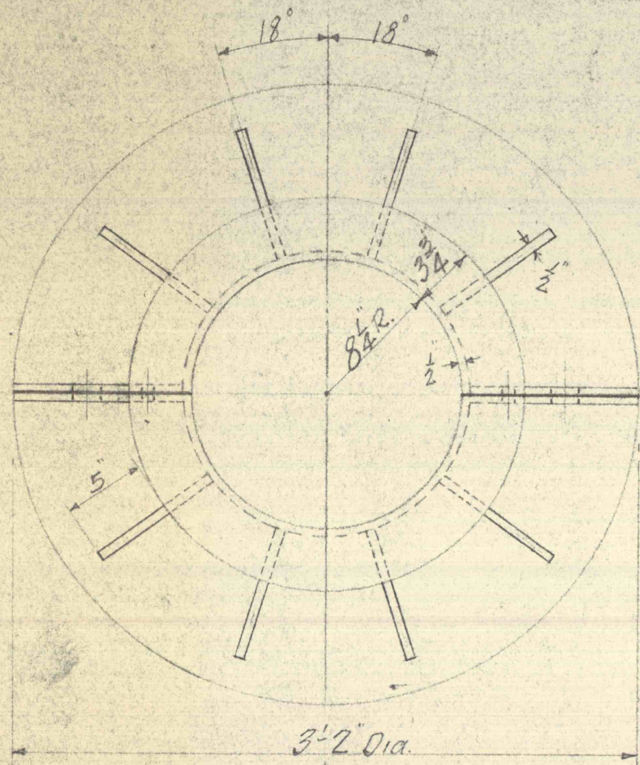
PLAN
