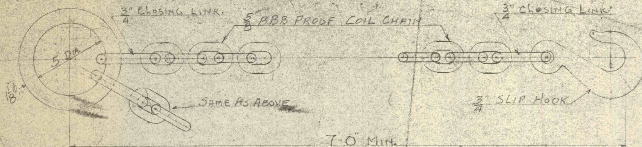
5/8" DOUBLE SLING CHAIN WITH RING AND SLIP HOOKS, ITEM #1.
