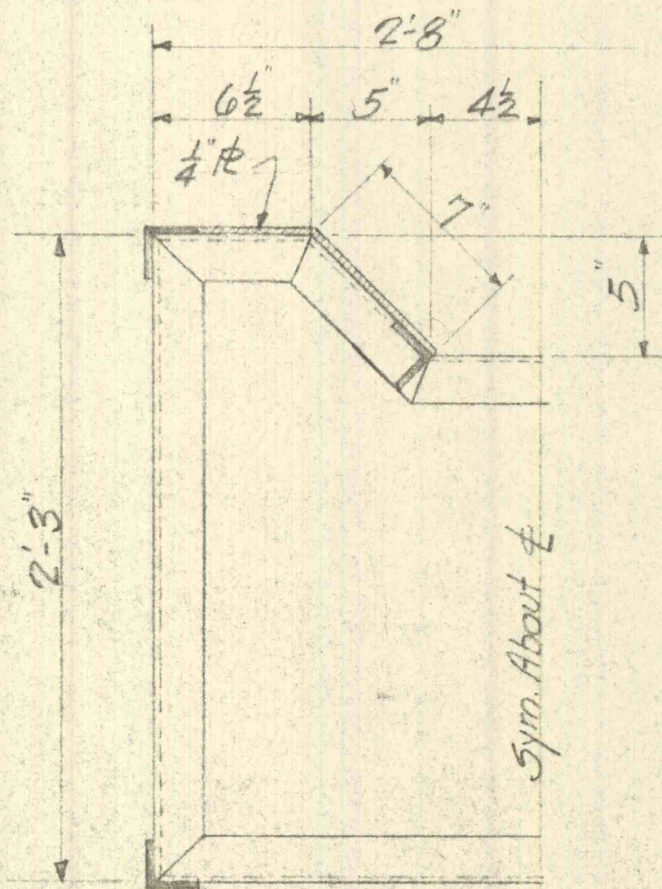
SECTION C-C
