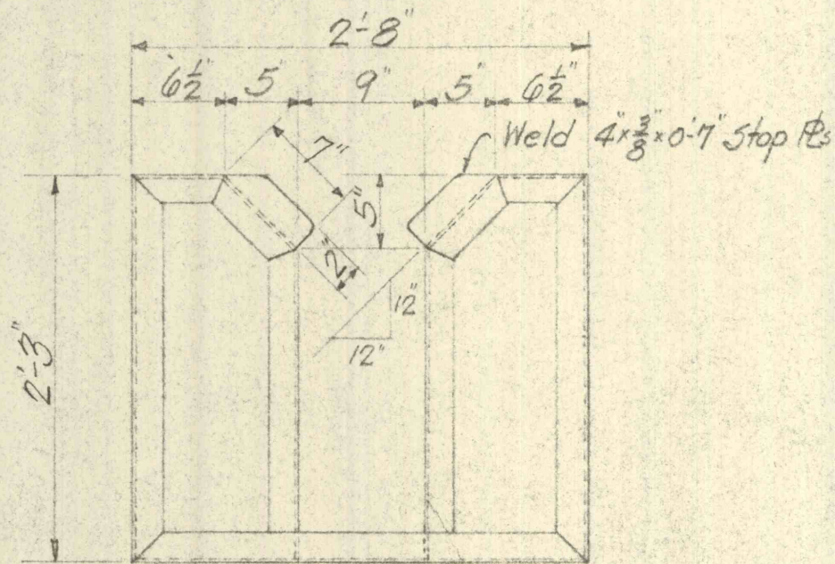
FRAME "B" 1-REQD
