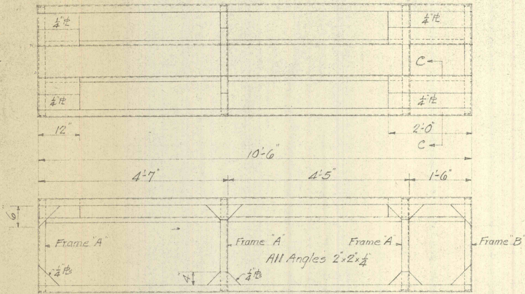
PIPE WORK BENCH ITEM #1
