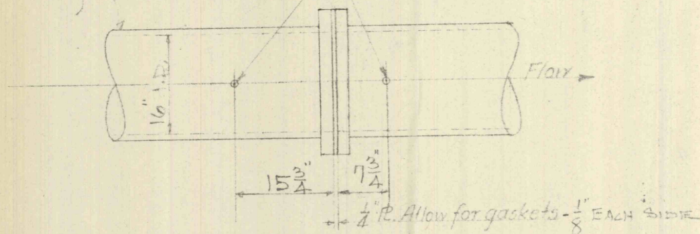
DIAGRAM FOR INSTALLING MANOMETER
