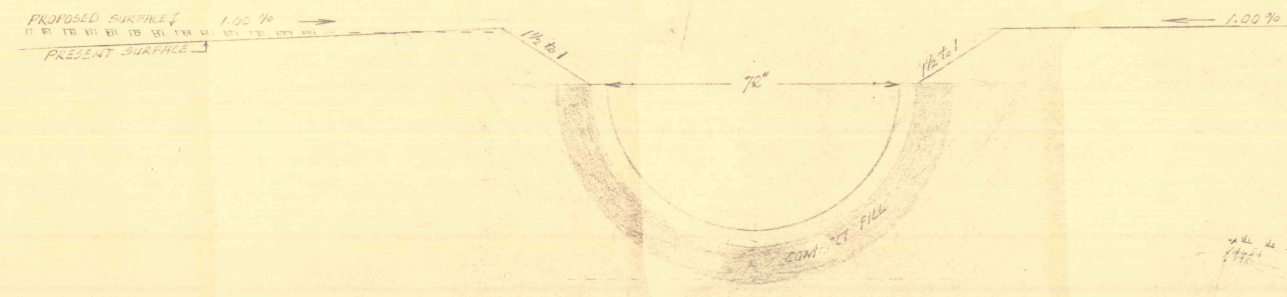
TYPICAL SECTION OF THE SEMI-CIRCLE CONCRETE FLUME FROM 0+00 EASTWARD TO 0+400 SCALE 8" = 1'
