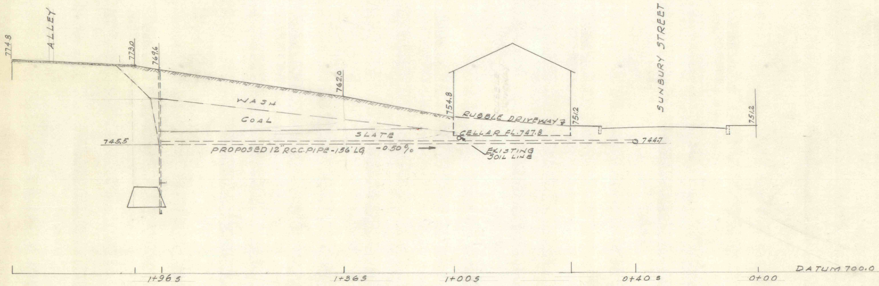
PROFILE B-B LOOKING WEST SCALE 1" = 20'
