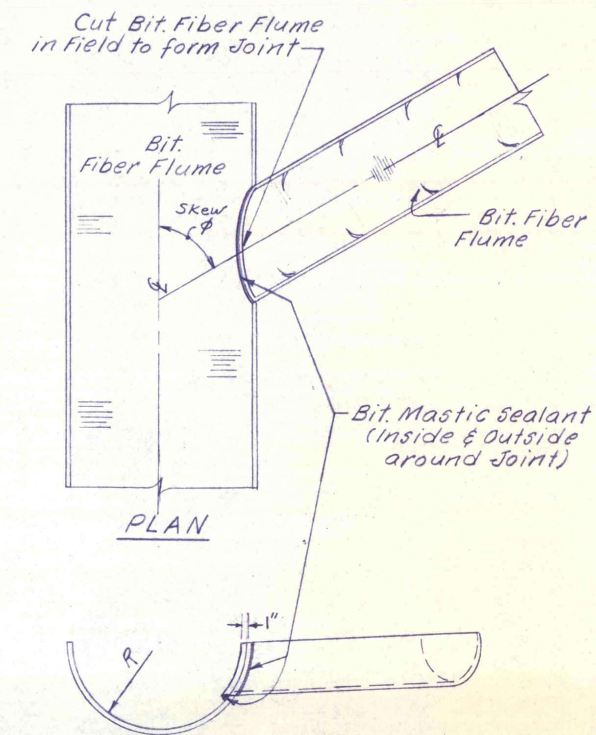
TYPICAL DETAIL FOR FLUME CONNECTIONS Scale 1" = 2'
