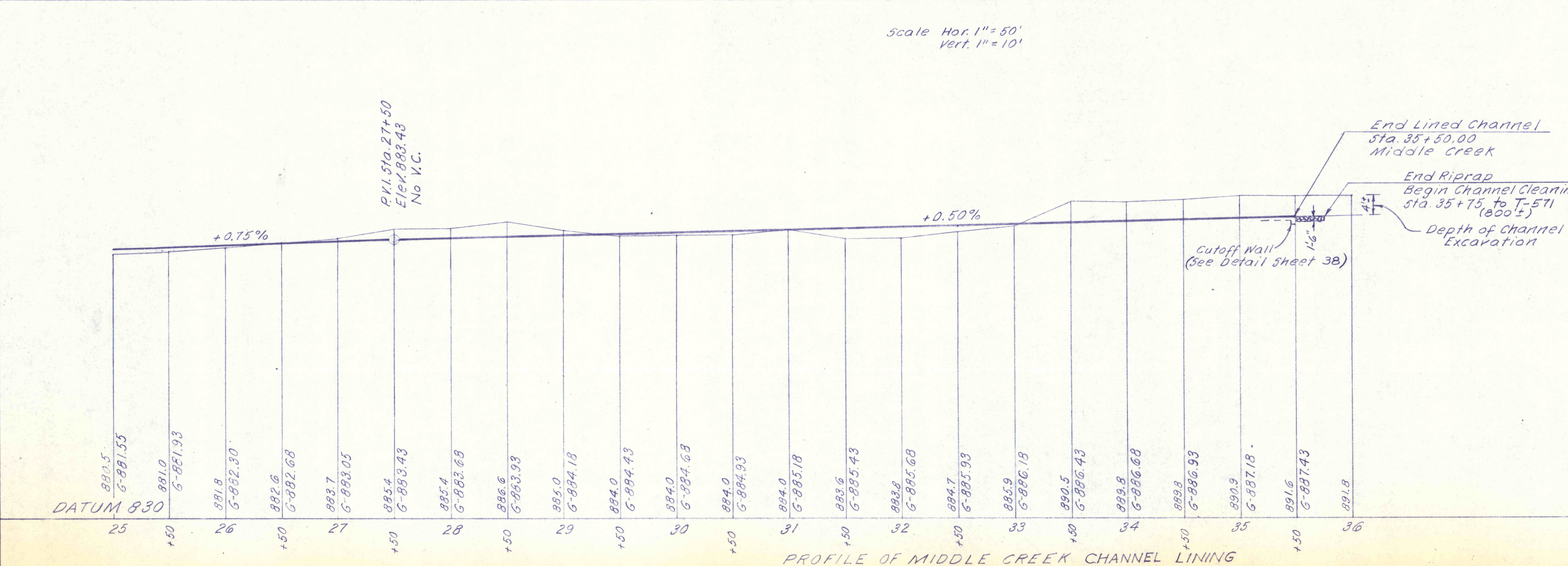
PROFILE OF MIDDLE CREEK CHANNEL LINING
