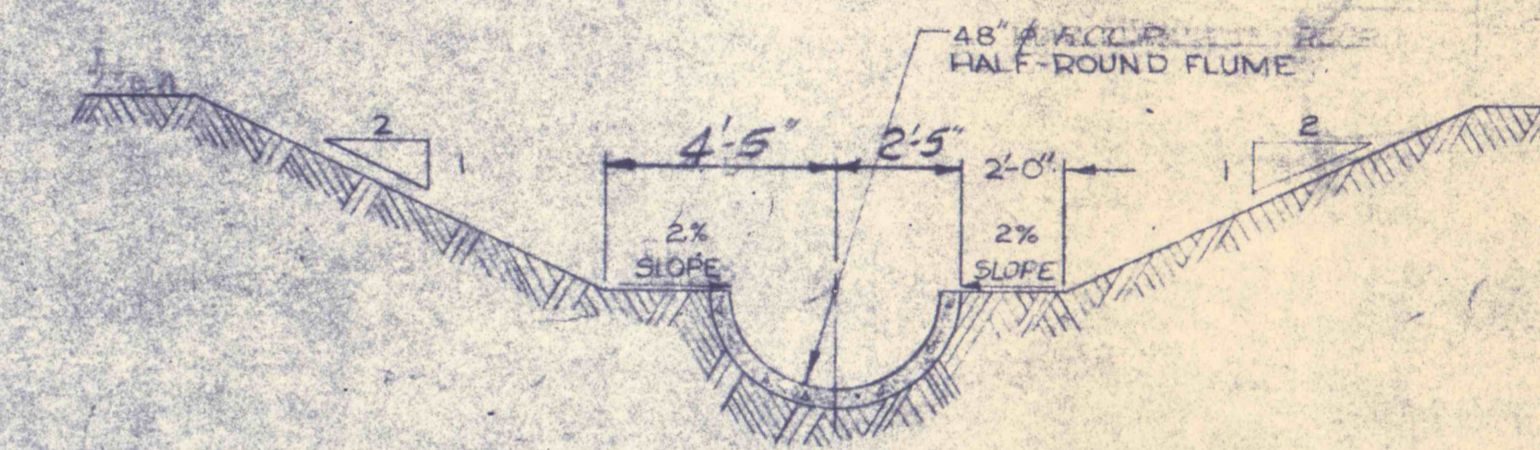
SECTION B-B SCALE 1/4" = 1'-0"
