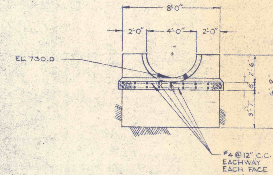
SECTION C-C SCALE 1/4" = 1'-0"
