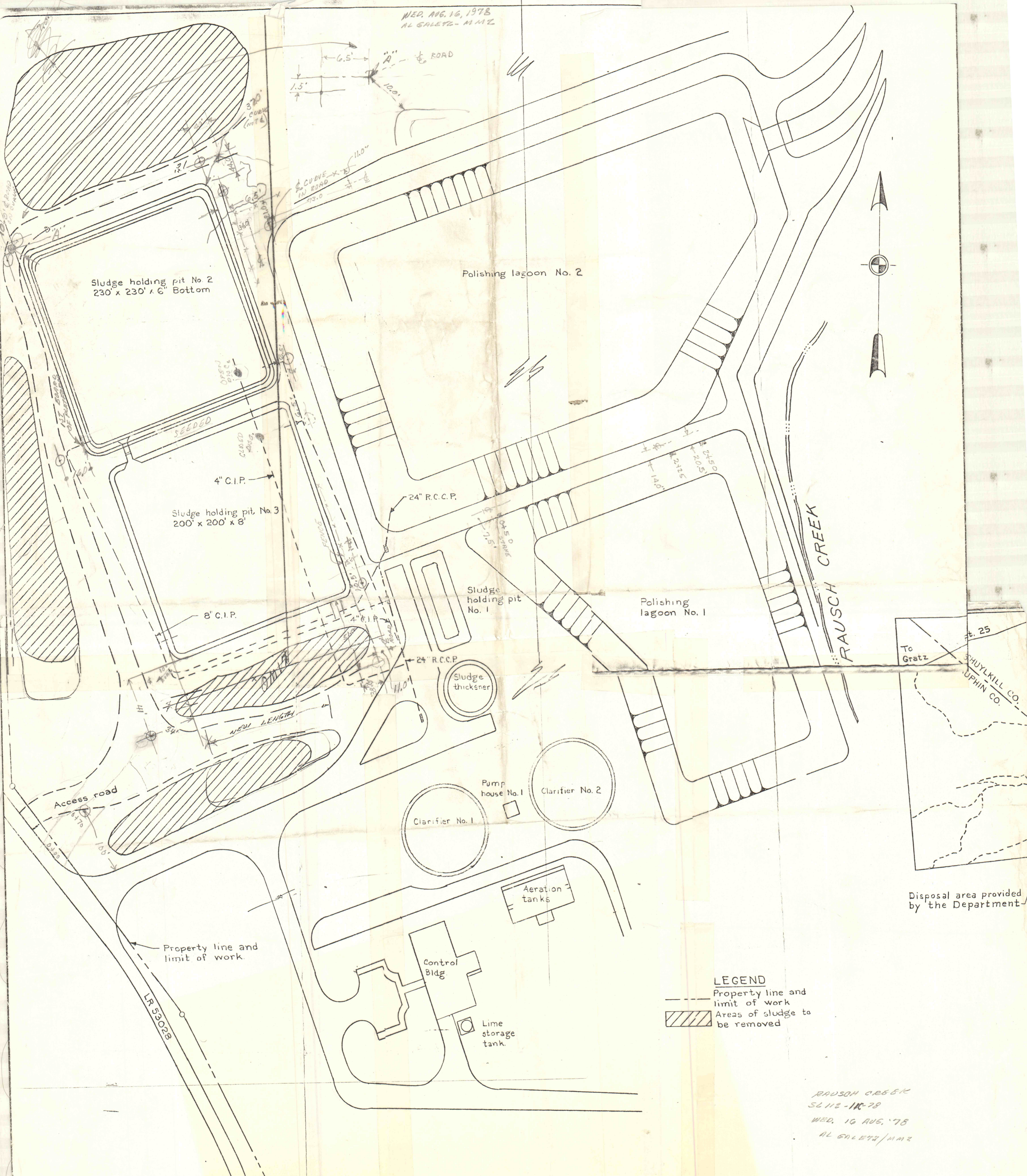
RAUSCH CREEK TREATMENT PLANT PLAN Scale: 1 in. = 50 ft.
