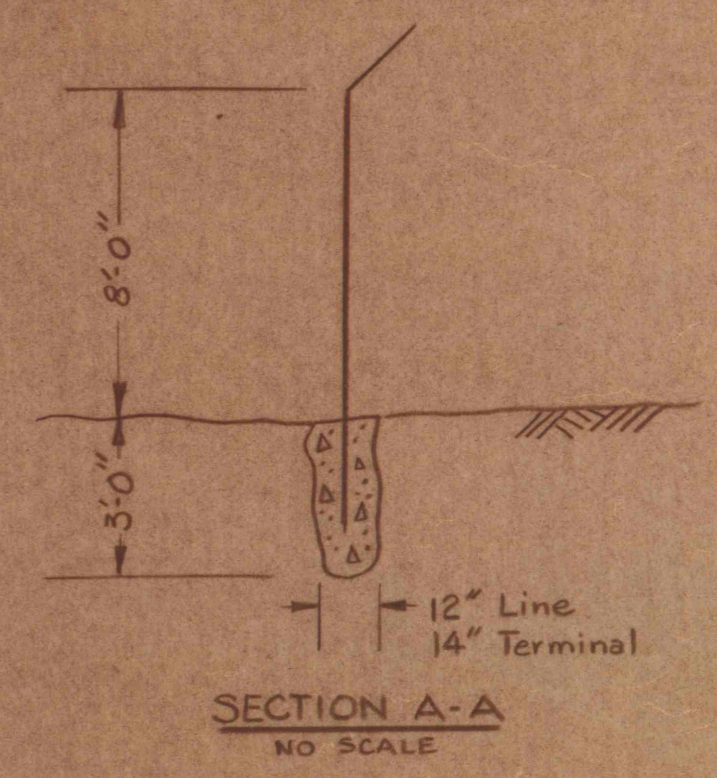
CHAIN LINK FENCE (See Notes and Technical Specification TS.5)
