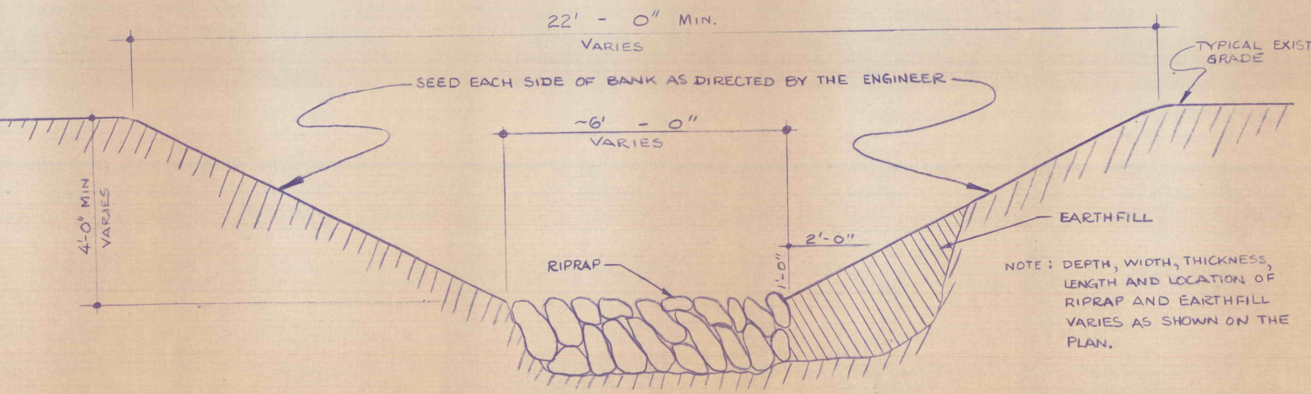
SECTION A-A TYPICAL CREEK CHANNEL RIPRAP AND EARTHFILL SCALE: 1/2" = 1'-0"
