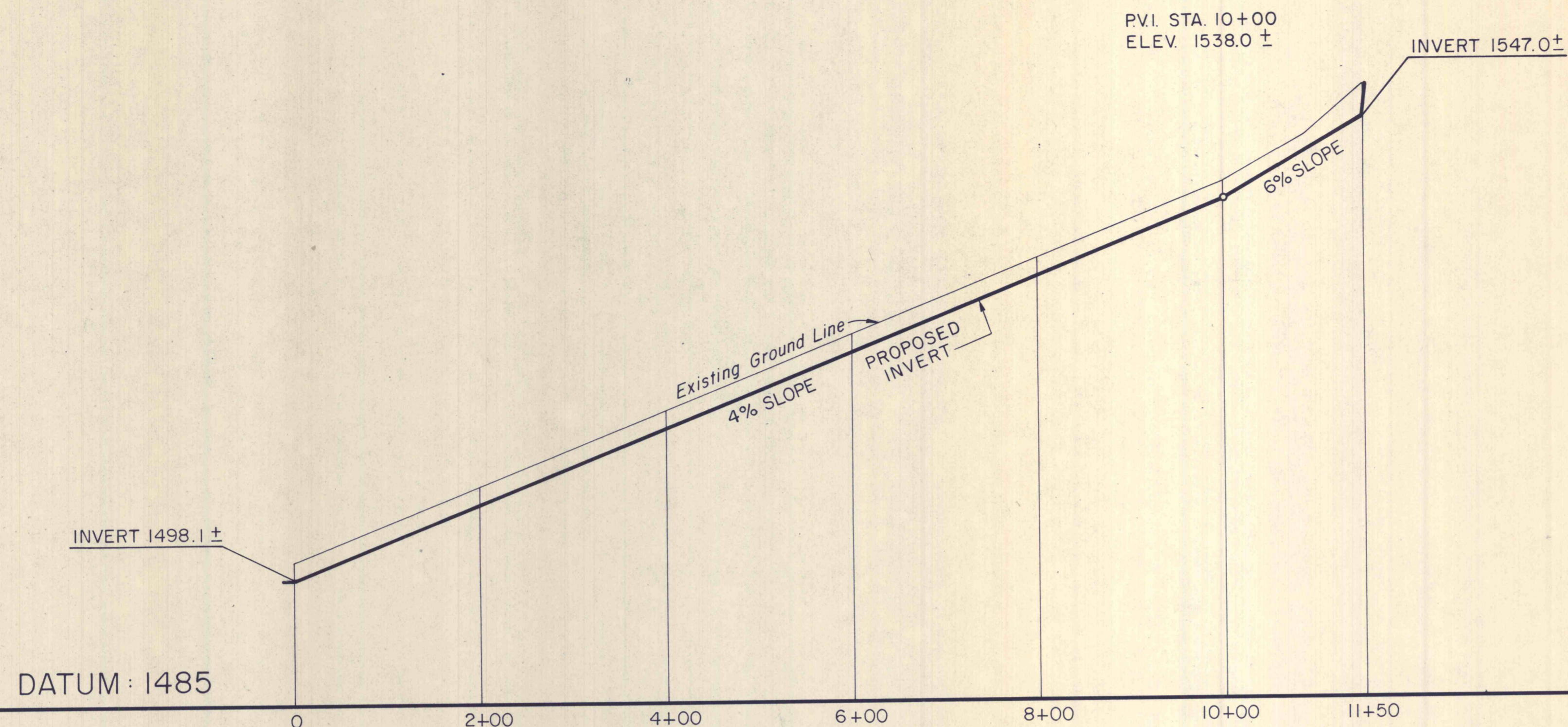
NORTHWEST DIVERSION DITCH OF EAST FLUME
