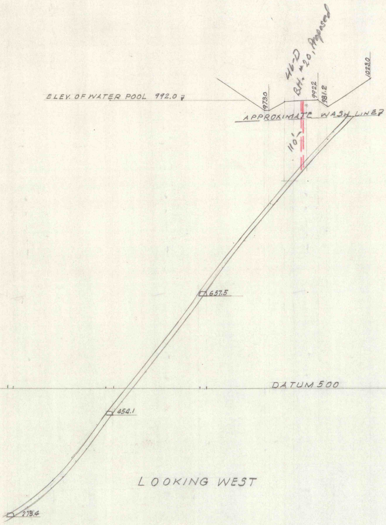
HAMMOND COLLIERY CROSS SECTION THROUGH No. 13 BREAST OFF WEST DIAMOND VEIN GWY.- 2ND LEVEL SCALE 1"=100' AUG. 1968
