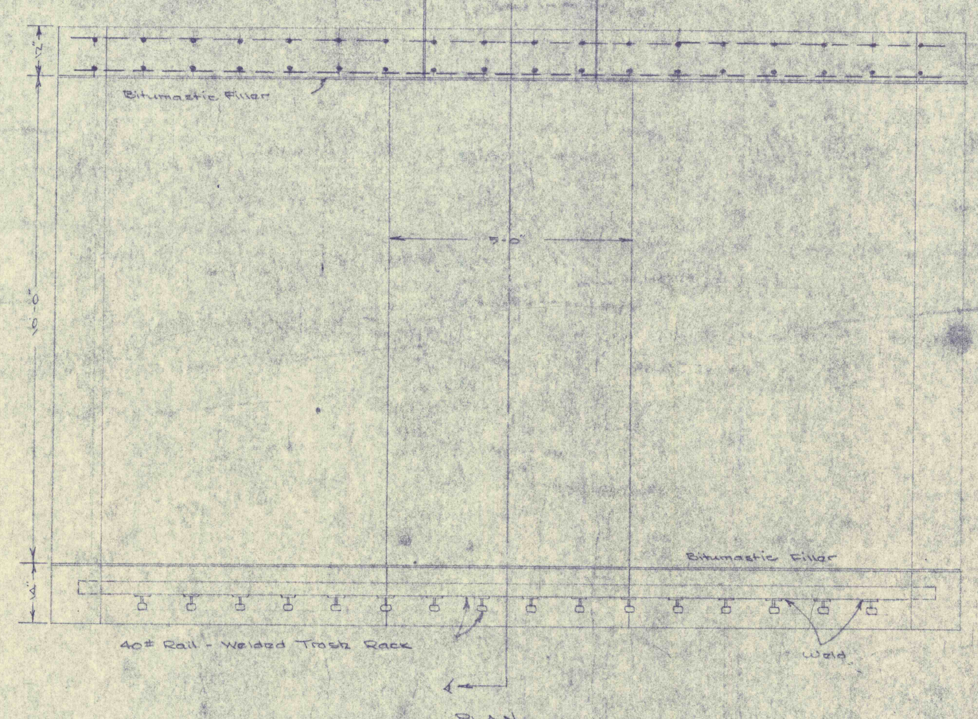
TRASH RACK AND INLET TO WALL FOUND CORRODED
