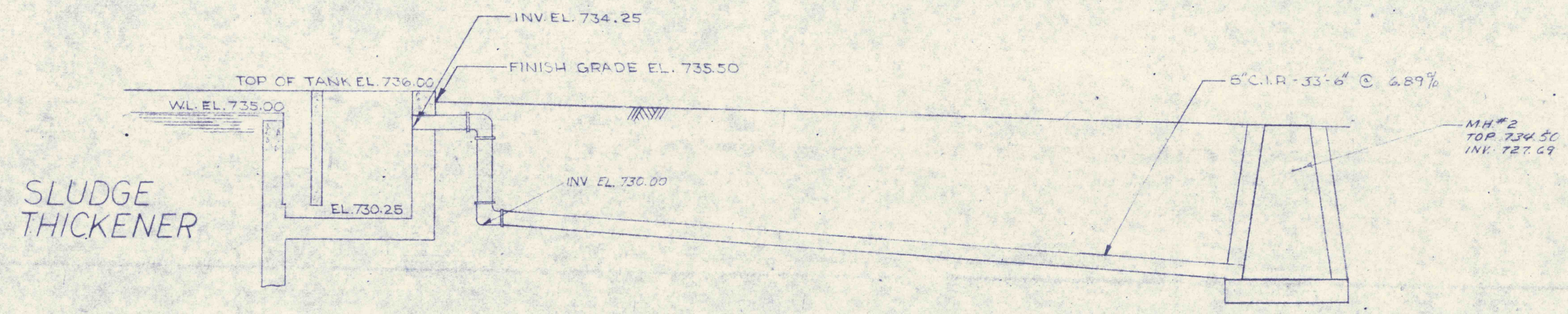
SECTION B-B DWG-C-4 & C-5 SCALE: 1/4" = 1'-0"
