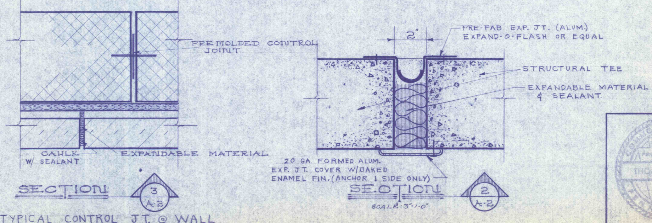
SECTION TYPICAL CONTROL JT. @ WALL
