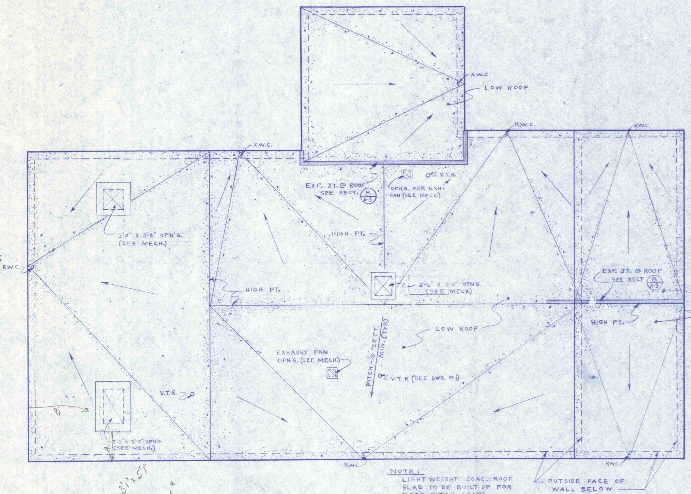
ROOF PLAN SCALE: 1/8" = 1'-0"
